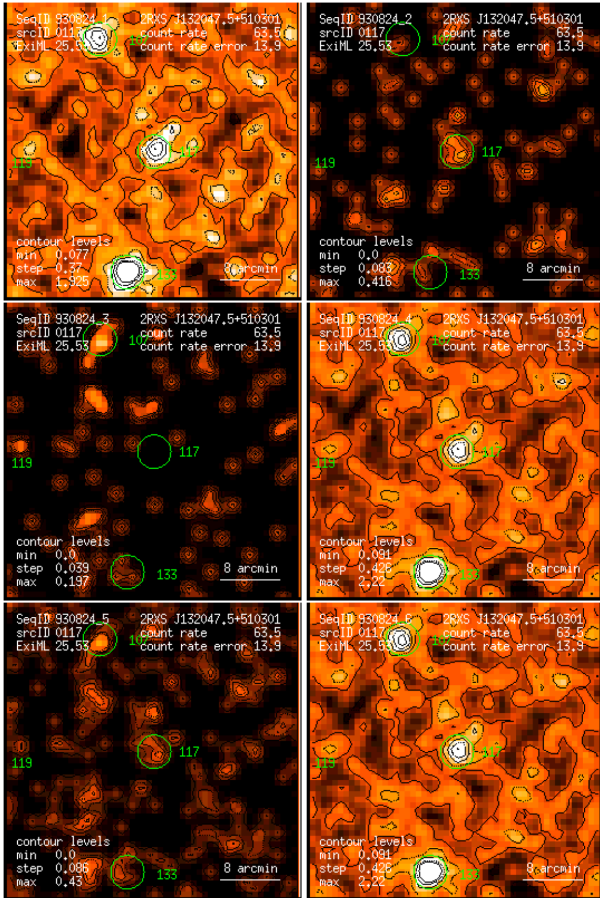
Figure 117: RASS 930824: detection 0117: band rate images, Gaussian filter: (1) PSPC channels 11 – 41, (2) 52 – 90, (3) 91 – 201, (4) 11 – 235, (5) 52 – 201, (6) 11 – 201. Broad band rates in counts/ks. Band rate contour levels in counts/ks/arcmin 2 .
