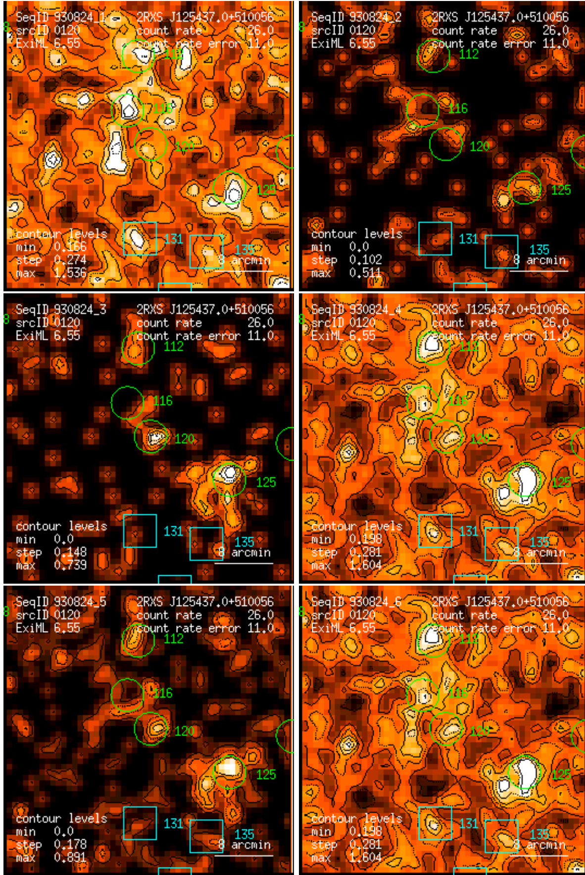
Figure 120: RASS 930824: detection 0120: band rate images, Gaussian filter: (1) PSPC channels 11 – 41, (2) 52 – 90, (3) 91 – 201, (4) 11 – 235, (5) 52 – 201, (6) 11 – 201. Broad band rates in counts/ks. Band rate contour levels in counts/ks/arcmin 2 .
