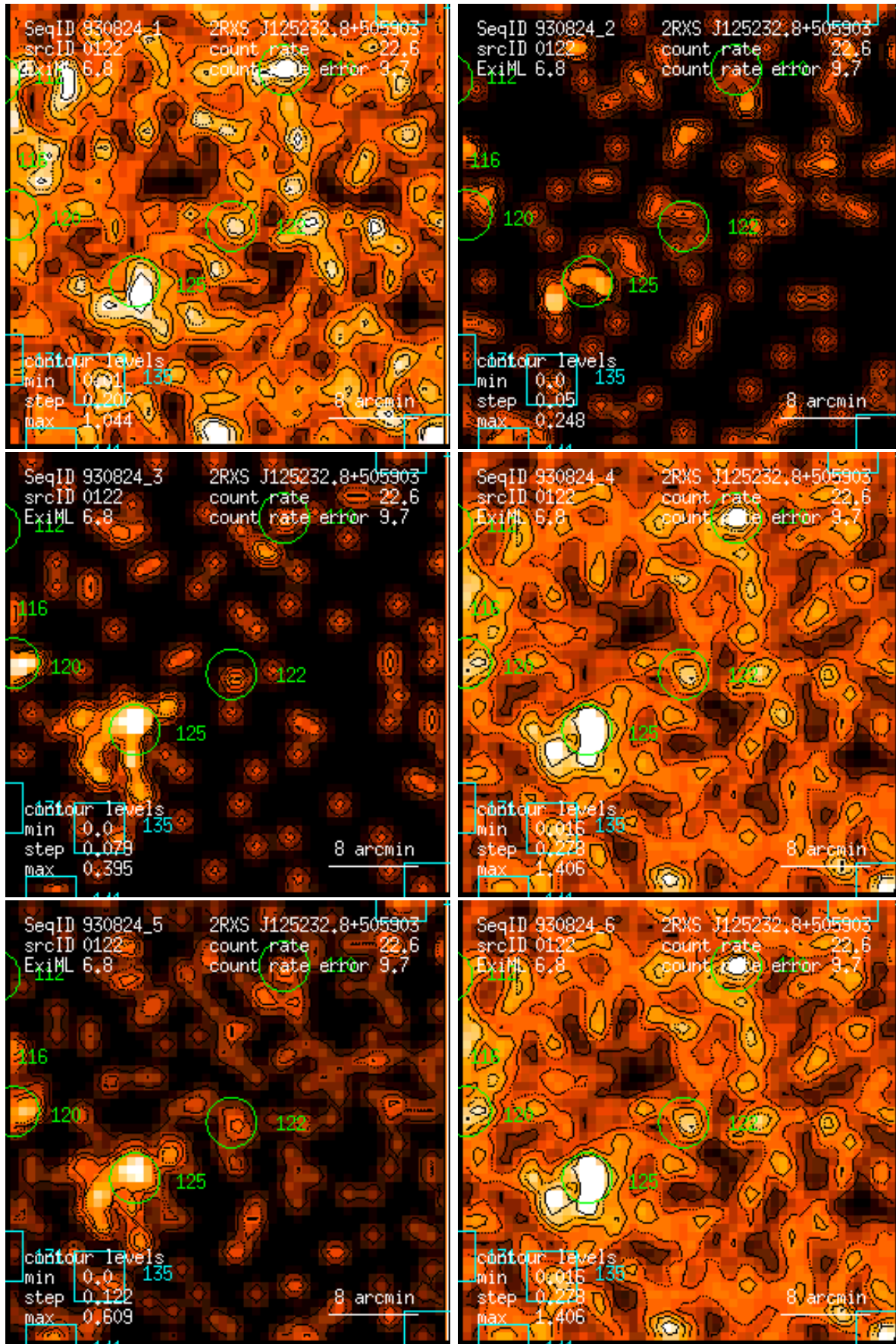
Figure 122: RASS 930824: detection 0122: band rate images, Gaussian filter: (1) PSPC channels 11 – 41, (2) 52 – 90, (3) 91 – 201, (4) 11 – 235, (5) 52 – 201, (6) 11 – 201. Broad band rates in counts/ks. Band rate contour levels in counts/ks/arcmin 2 .
