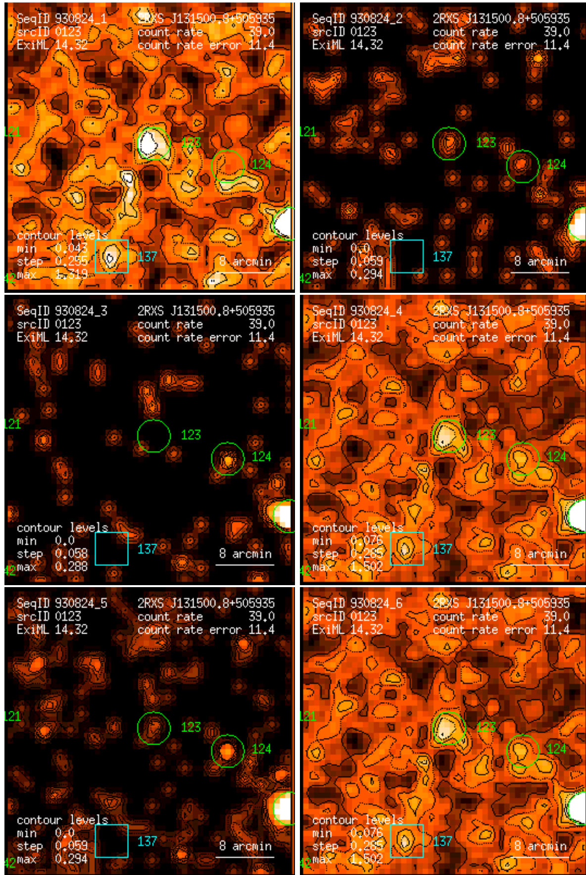
Figure 123: RASS 930824: detection 0123: band rate images, Gaussian filter: (1) PSPC channels 11 – 41, (2) 52 – 90, (3) 91 – 201, (4) 11 – 235, (5) 52 – 201, (6) 11 – 201. Broad band rates in counts/ks. Band rate contour levels in counts/ks/arcmin 2 .
