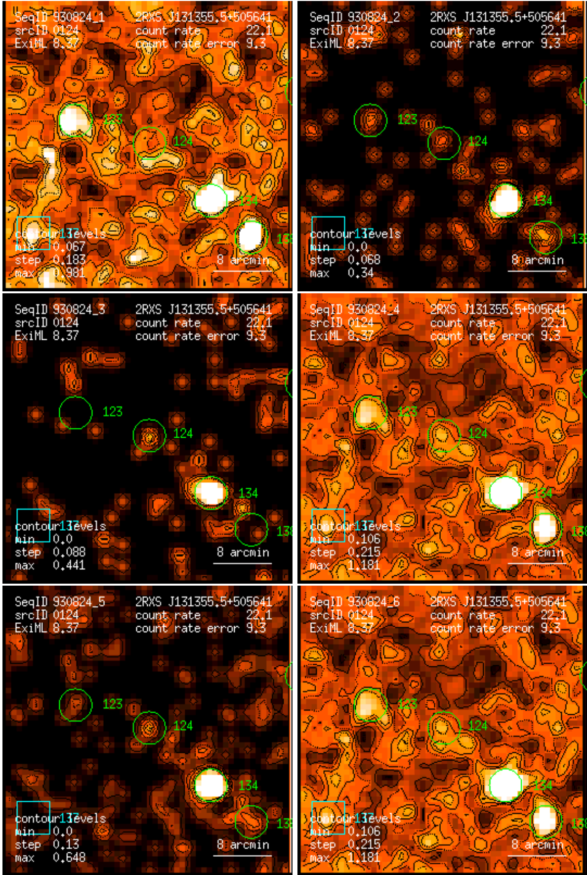
Figure 124: RASS 930824: detection 0124: band rate images, Gaussian filter: (1) PSPC channels 11 – 41, (2) 52 – 90, (3) 91 – 201, (4) 11 – 235, (5) 52 – 201, (6) 11 – 201. Broad band rates in counts/ks. Band rate contour levels in counts/ks/arcmin 2 .
