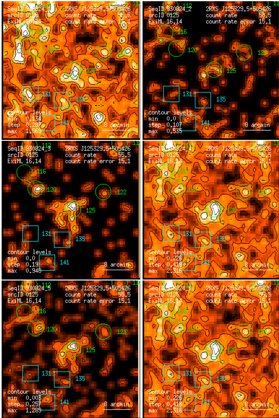
Figure 125: RASS 930824: detection 0125: band rate images, Gaussian filter: (1) PSPC channels 11 – 41, (2) 52 – 90, (3) 91 – 201, (4) 11 – 235, (5) 52 – 201, (6) 11 – 201. Broad band rates in counts/ks. Band rate contour levels in counts/ks/arcmin 2 .
