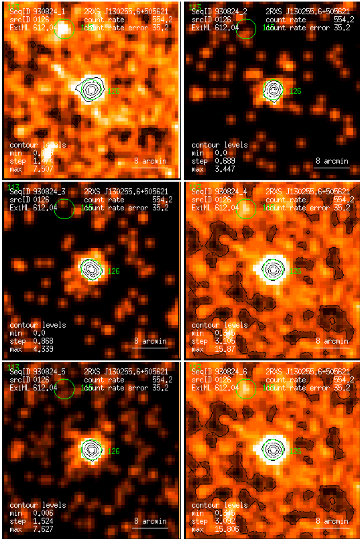
Figure 126: RASS 930824: detection 0126: band rate images, Gaussian filter: (1) PSPC channels 11 – 41, (2) 52 – 90, (3) 91 – 201, (4) 11 – 235, (5) 52 – 201, (6) 11 – 201. Broad band rates in counts/ks. Band rate contour levels in counts/ks/arcmin 2 .
