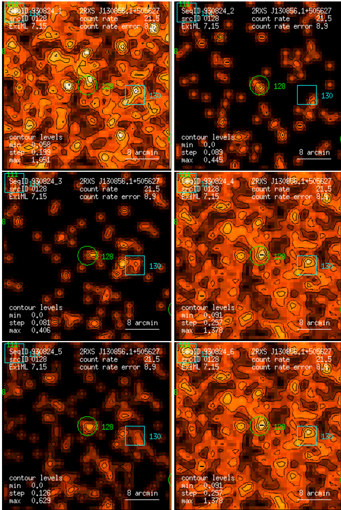
Figure 128: RASS 930824: detection 0128: band rate images, Gaussian filter: (1) PSPC channels 11 – 41, (2) 52 – 90, (3) 91 – 201, (4) 11 – 235, (5) 52 – 201, (6) 11 – 201. Broad band rates in counts/ks. Band rate contour levels in counts/ks/arcmin 2 .
