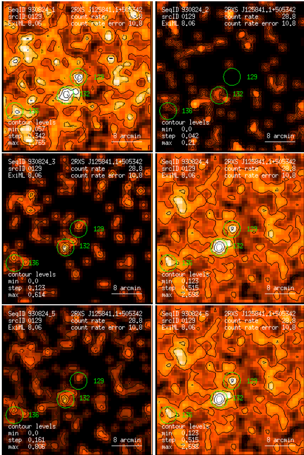
Figure 129: RASS 930824: detection 0129: band rate images, Gaussian filter: (1) PSPC channels 11 – 41, (2) 52 – 90, (3) 91 – 201, (4) 11 – 235, (5) 52 – 201, (6) 11 – 201. Broad band rates in counts/ks. Band rate contour levels in counts/ks/arcmin 2 .
