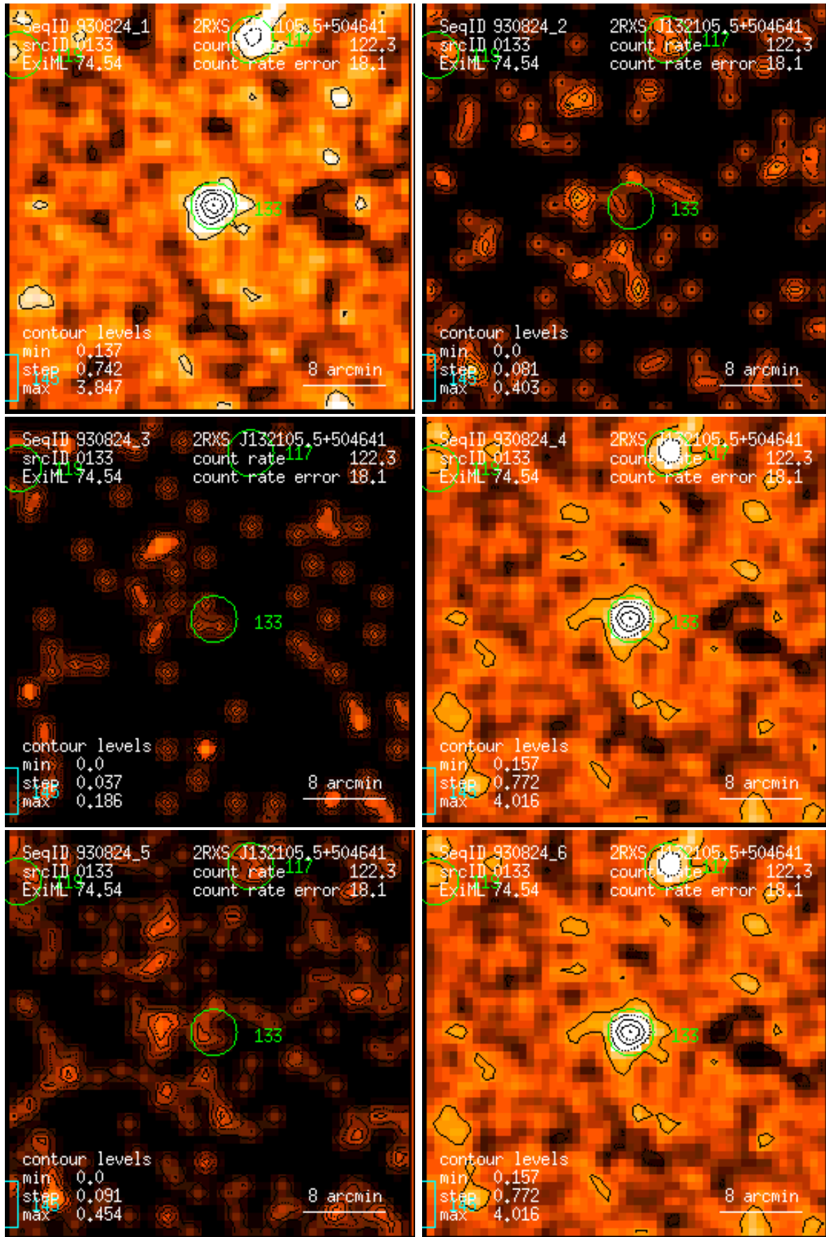
Figure 133: RASS 930824: detection 0133: band rate images, Gaussian filter: (1) PSPC channels 11 – 41, (2) 52 – 90, (3) 91 – 201, (4) 11 – 235, (5) 52 – 201, (6) 11 – 201. Broad band rates in counts/ks. Band rate contour levels in counts/ks/arcmin 2 .
