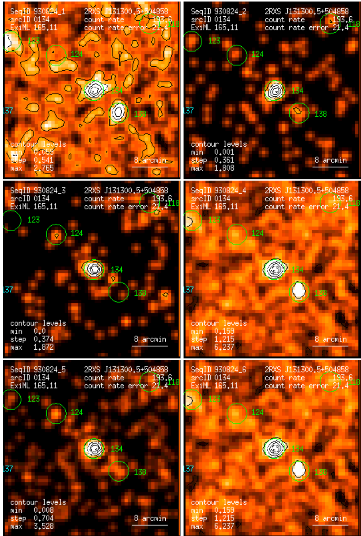
Figure 134: RASS 930824: detection 0134: band rate images, Gaussian filter: (1) PSPC channels 11 – 41, (2) 52 – 90, (3) 91 – 201, (4) 11 – 235, (5) 52 – 201, (6) 11 – 201. Broad band rates in counts/ks. Band rate contour levels in counts/ks/arcmin 2 .
