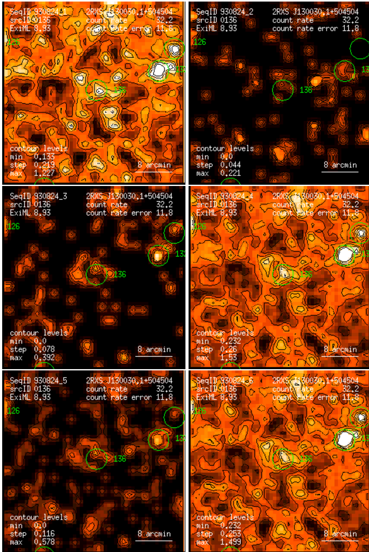
Figure 136: RASS 930824: detection 0136: band rate images, Gaussian filter: (1) PSPC channels 11 – 41, (2) 52 – 90, (3) 91 – 201, (4) 11 – 235, (5) 52 – 201, (6) 11 – 201. Broad band rates in counts/ks. Band rate contour levels in counts/ks/arcmin 2 .
