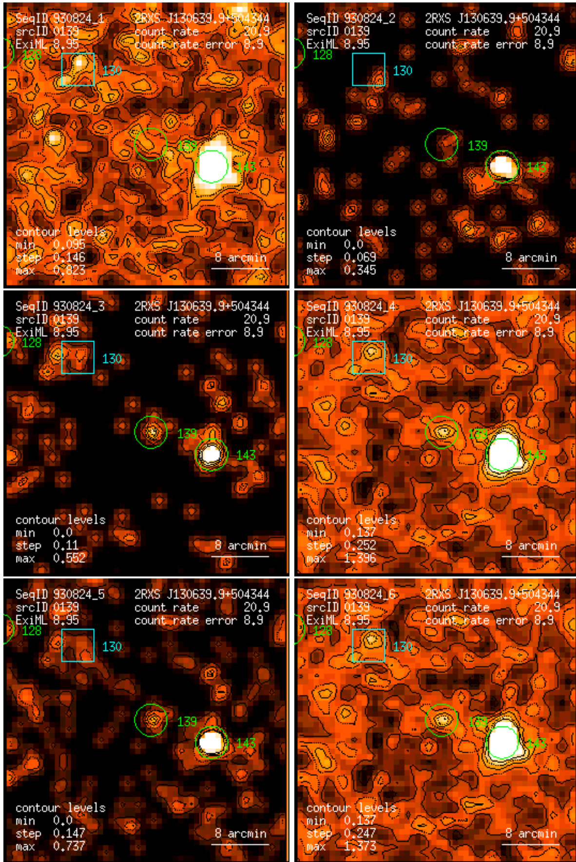
Figure 139: RASS 930824: detection 0139: band rate images, Gaussian filter: (1) PSPC channels 11 – 41, (2) 52 – 90, (3) 91 – 201, (4) 11 – 235, (5) 52 – 201, (6) 11 – 201. Broad band rates in counts/ks. Band rate contour levels in counts/ks/arcmin 2 .
