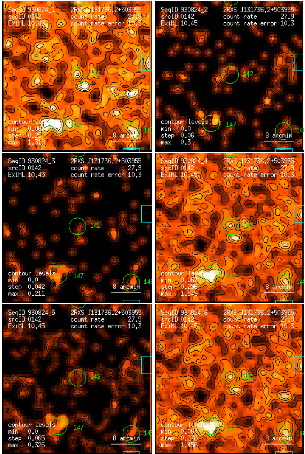
Figure 142: RASS 930824: detection 0142: band rate images, Gaussian filter: (1) PSPC channels 11 – 41, (2) 52 – 90, (3) 91 – 201, (4) 11 – 235, (5) 52 – 201, (6) 11 – 201. Broad band rates in counts/ks. Band rate contour levels in counts/ks/arcmin 2 .
