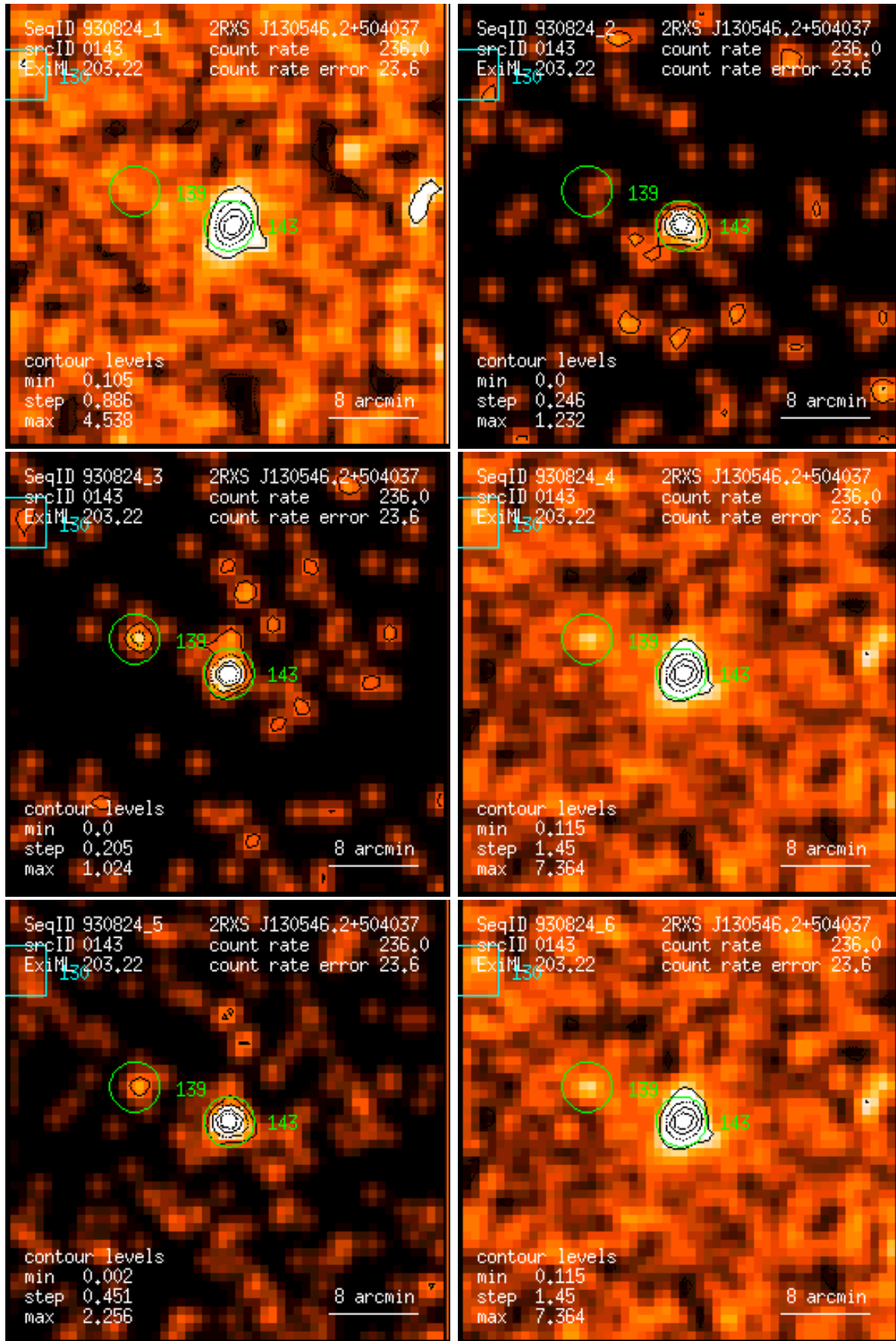
Figure 143: RASS 930824: detection 0143: band rate images, Gaussian filter: (1) PSPC channels 11 – 41, (2) 52 – 90, (3) 91 – 201, (4) 11 – 235, (5) 52 – 201, (6) 11 – 201. Broad band rates in counts/ks. Band rate contour levels in counts/ks/arcmin 2 .
