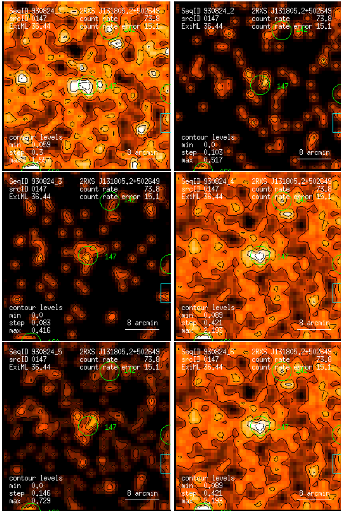
Figure 147: RASS 930824: detection 0147: band rate images, Gaussian filter: (1) PSPC channels 11 – 41, (2) 52 – 90, (3) 91 – 201, (4) 11 – 235, (5) 52 – 201, (6) 11 – 201. Broad band rates in counts/ks. Band rate contour levels in counts/ks/arcmin 2 .
