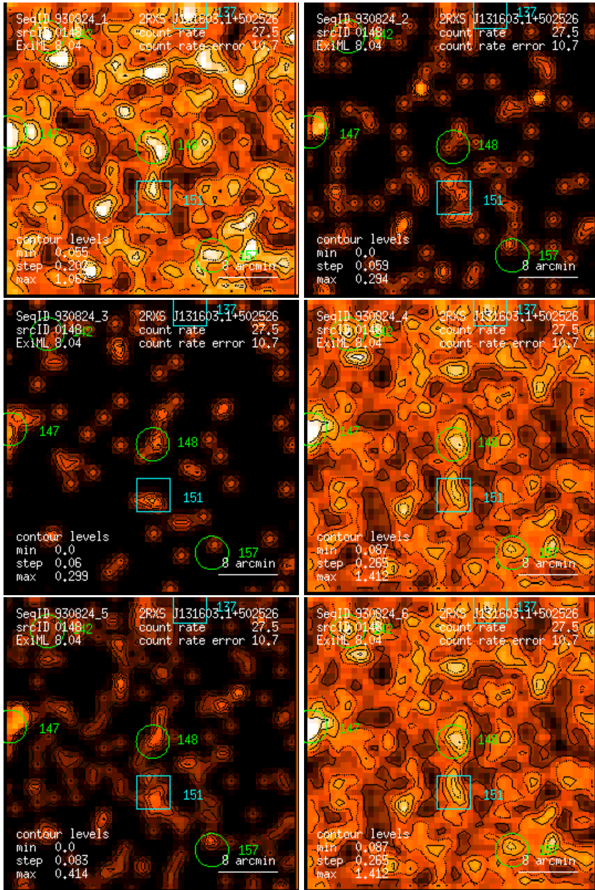
Figure 148: RASS 930824: detection 0148: band rate images, Gaussian filter: (1) PSPC channels 11 – 41, (2) 52 – 90, (3) 91 – 201, (4) 11 – 235, (5) 52 – 201, (6) 11 – 201. Broad band rates in counts/ks. Band rate contour levels in counts/ks/arcmin 2 .
