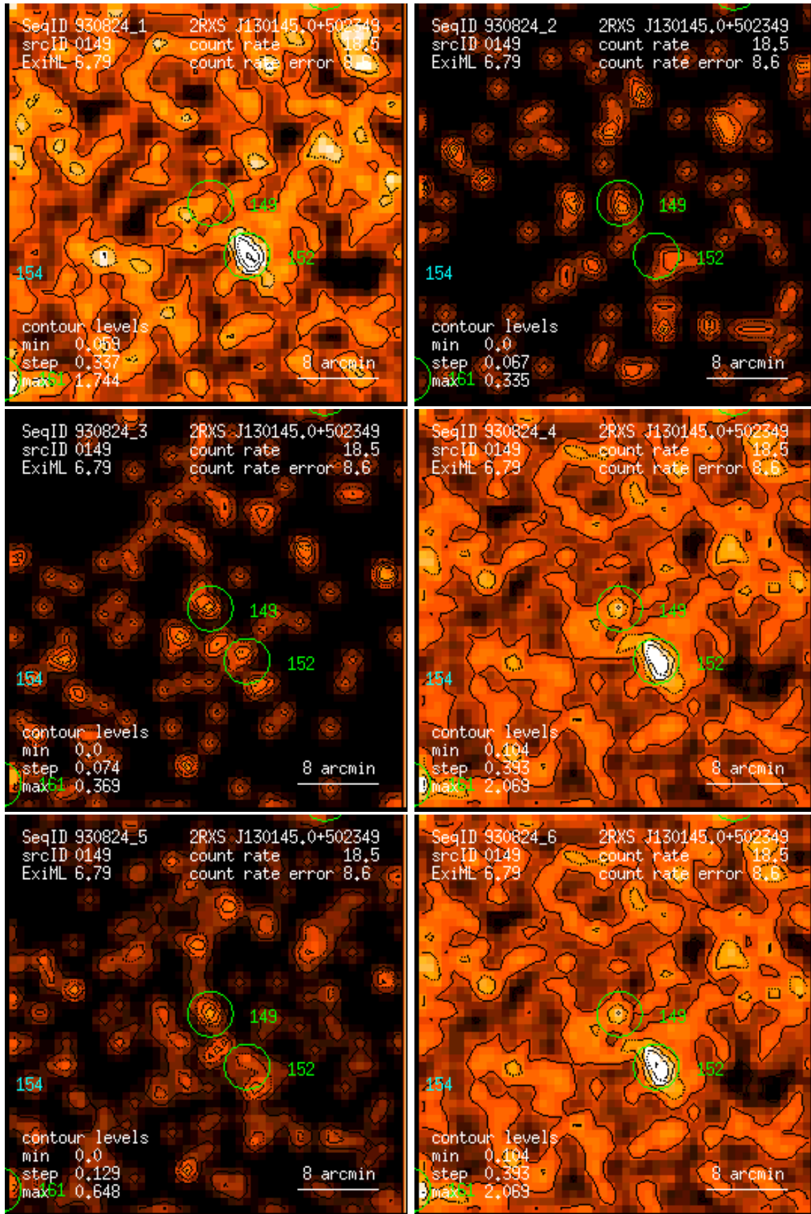
Figure 149: RASS 930824: detection 0149: band rate images, Gaussian filter: (1) PSPC channels 11 – 41, (2) 52 – 90, (3) 91 – 201, (4) 11 – 235, (5) 52 – 201, (6) 11 – 201. Broad band rates in counts/ks. Band rate contour levels in counts/ks/arcmin 2 .
