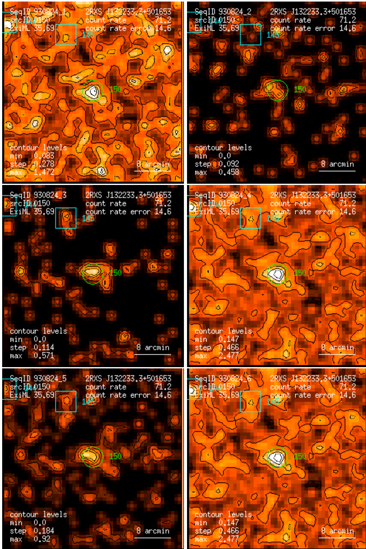
Figure 150: RASS 930824: detection 0150: band rate images, Gaussian filter: (1) PSPC channels 11 – 41, (2) 52 – 90, (3) 91 – 201, (4) 11 – 235, (5) 52 – 201, (6) 11 – 201. Broad band rates in counts/ks. Band rate contour levels in counts/ks/arcmin 2 .
