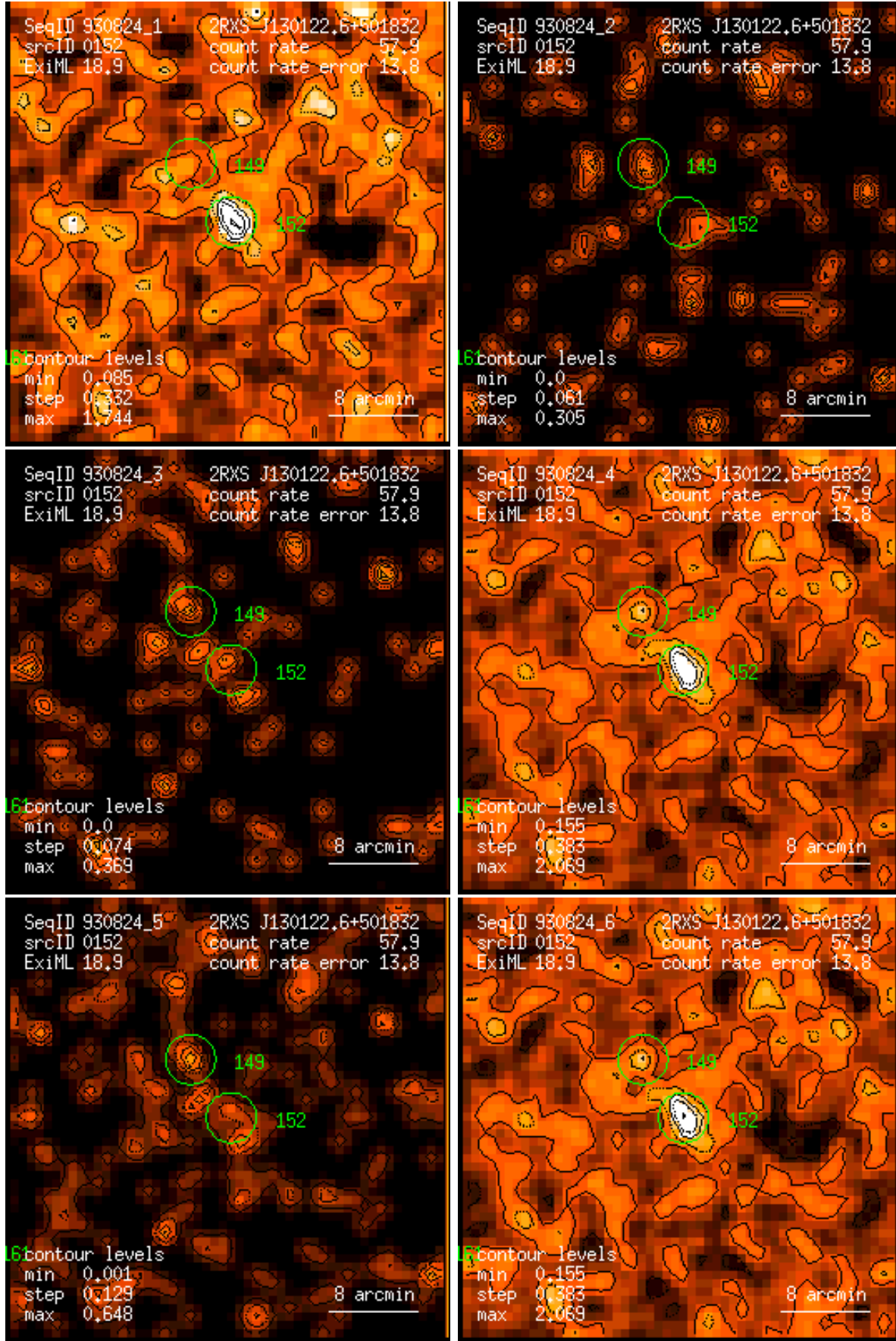
Figure 152: RASS 930824: detection 0152: band rate images, Gaussian filter: (1) PSPC channels 11 – 41, (2) 52 – 90, (3) 91 – 201, (4) 11 – 235, (5) 52 – 201, (6) 11 – 201. Broad band rates in counts/ks. Band rate contour levels in counts/ks/arcmin 2 .
