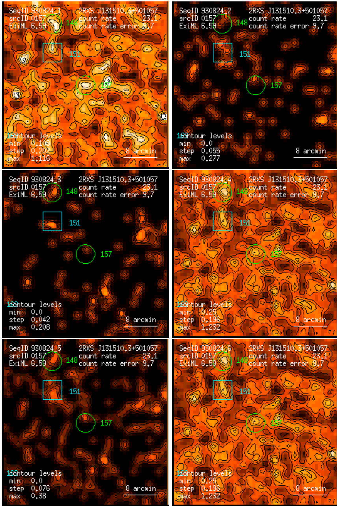
Figure 157: RASS 930824: detection 0157: band rate images, Gaussian filter: (1) PSPC channels 11 – 41, (2) 52 – 90, (3) 91 – 201, (4) 11 – 235, (5) 52 – 201, (6) 11 – 201. Broad band rates in counts/ks. Band rate contour levels in counts/ks/arcmin 2 .
