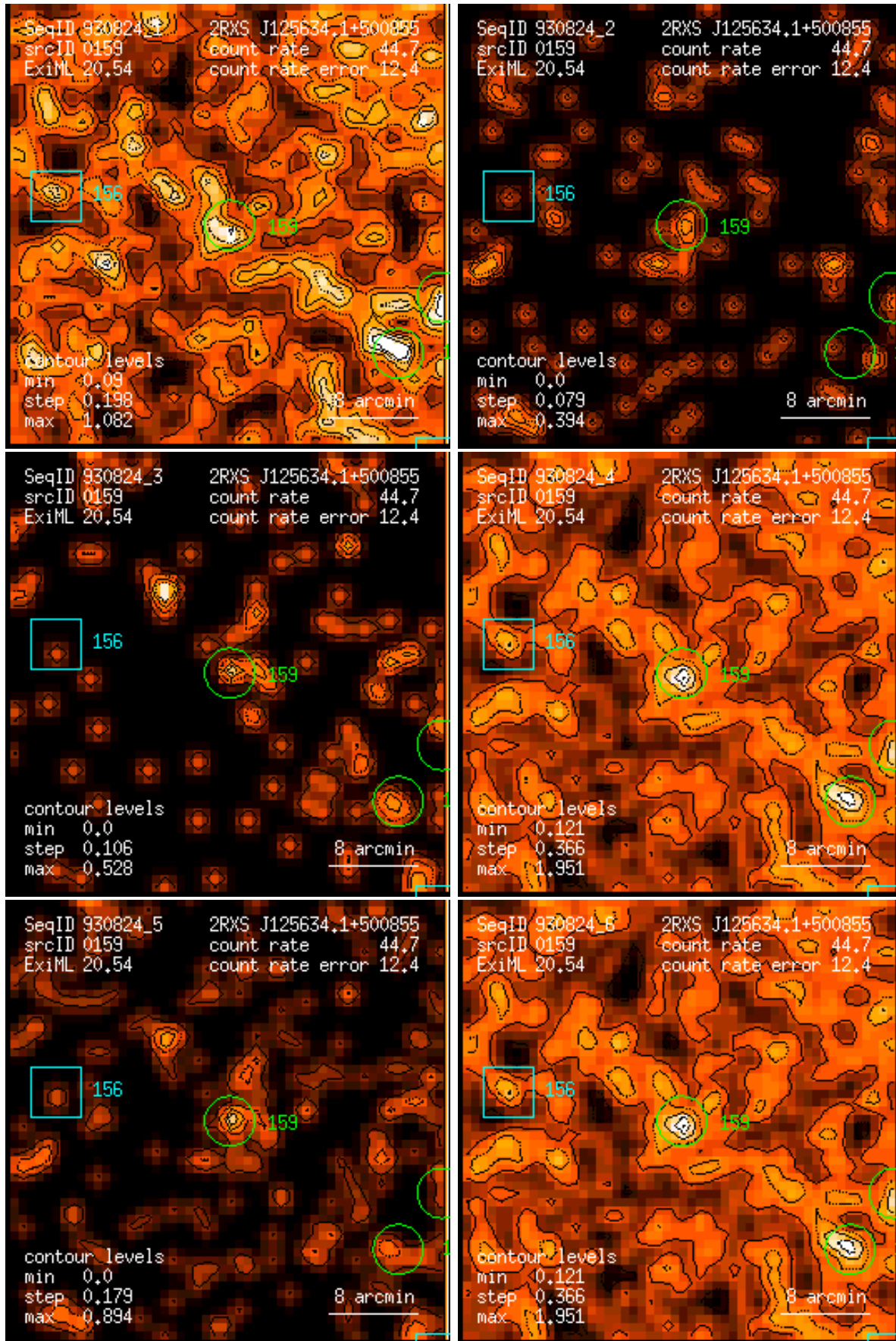
Figure 159: RASS 930824: detection 0159: band rate images, Gaussian filter: (1) PSPC channels 11 – 41, (2) 52 – 90, (3) 91 – 201, (4) 11 – 235, (5) 52 – 201, (6) 11 – 201. Broad band rates in counts/ks. Band rate contour levels in counts/ks/arcmin 2 .
