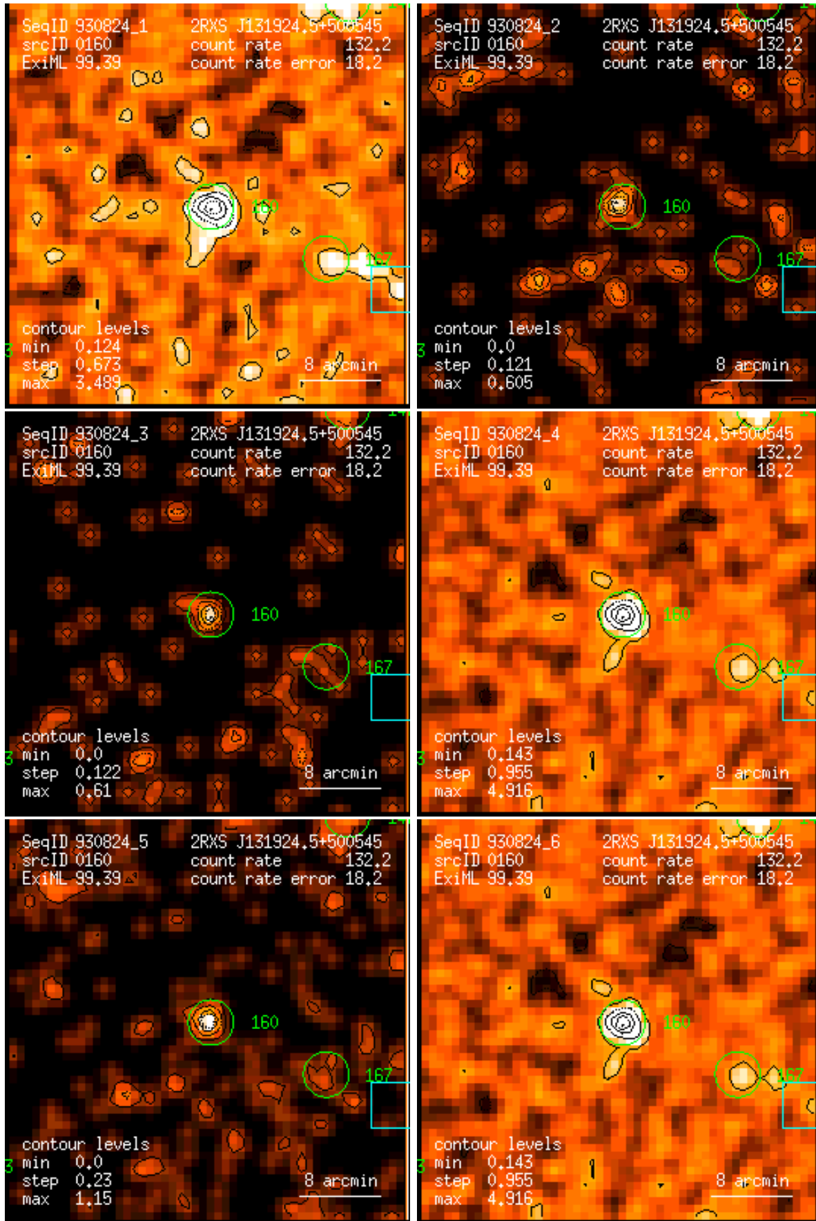
Figure 160: RASS 930824: detection 0160: band rate images, Gaussian filter: (1) PSPC channels 11 – 41, (2) 52 – 90, (3) 91 – 201, (4) 11 – 235, (5) 52 – 201, (6) 11 – 201. Broad band rates in counts/ks. Band rate contour levels in counts/ks/arcmin 2 .
