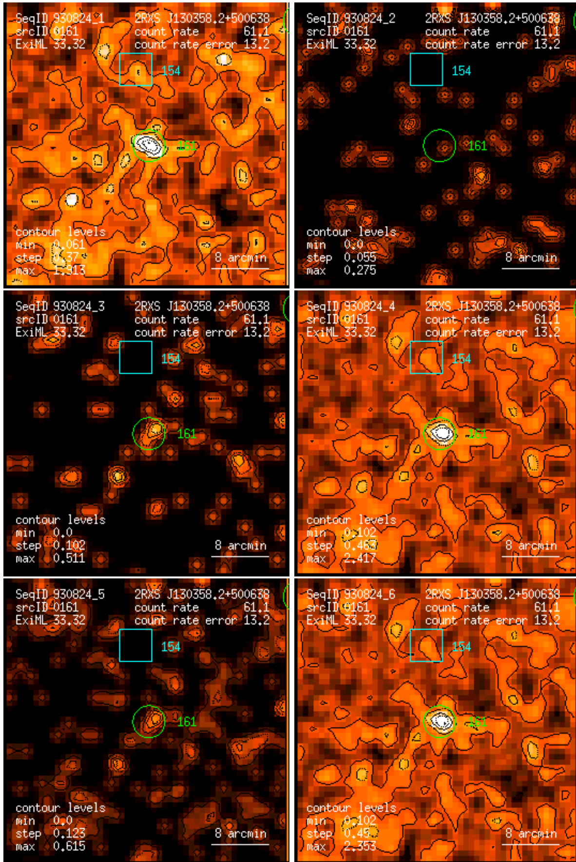
Figure 161: RASS 930824: detection 0161: band rate images, Gaussian filter: (1) PSPC channels 11 – 41, (2) 52 – 90, (3) 91 – 201, (4) 11 – 235, (5) 52 – 201, (6) 11 – 201. Broad band rates in counts/ks. Band rate contour levels in counts/ks/arcmin 2 .
