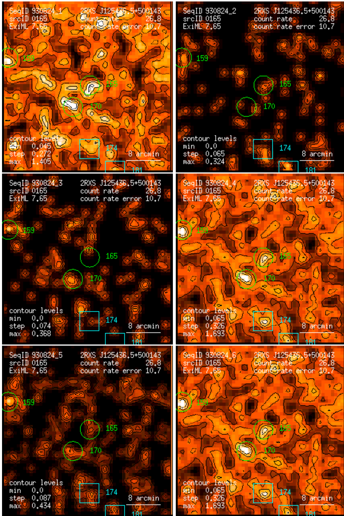
Figure 165: RASS 930824: detection 0165: band rate images, Gaussian filter: (1) PSPC channels 11 – 41, (2) 52 – 90, (3) 91 – 201, (4) 11 – 235, (5) 52 – 201, (6) 11 – 201. Broad band rates in counts/ks. Band rate contour levels in counts/ks/arcmin 2 .
