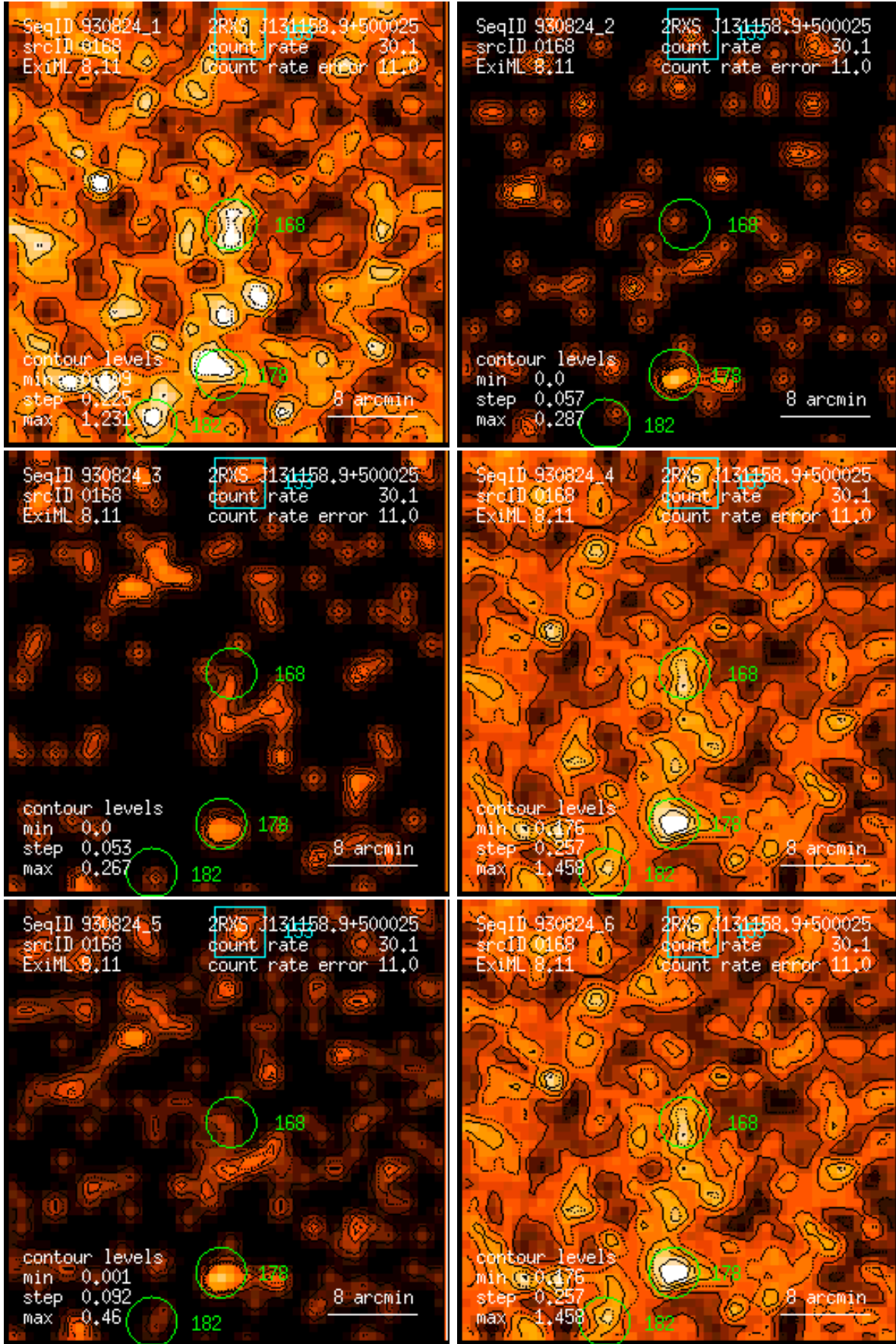
Figure 168: RASS 930824: detection 0168: band rate images, Gaussian filter: (1) PSPC channels 11 – 41, (2) 52 – 90, (3) 91 – 201, (4) 11 – 235, (5) 52 – 201, (6) 11 – 201. Broad band rates in counts/ks. Band rate contour levels in counts/ks/arcmin 2 .
