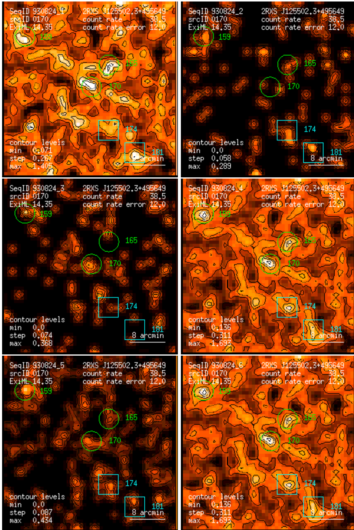
Figure 170: RASS 930824: detection 0170: band rate images, Gaussian filter: (1) PSPC channels 11 – 41, (2) 52 – 90, (3) 91 – 201, (4) 11 – 235, (5) 52 – 201, (6) 11 – 201. Broad band rates in counts/ks. Band rate contour levels in counts/ks/arcmin 2 .
