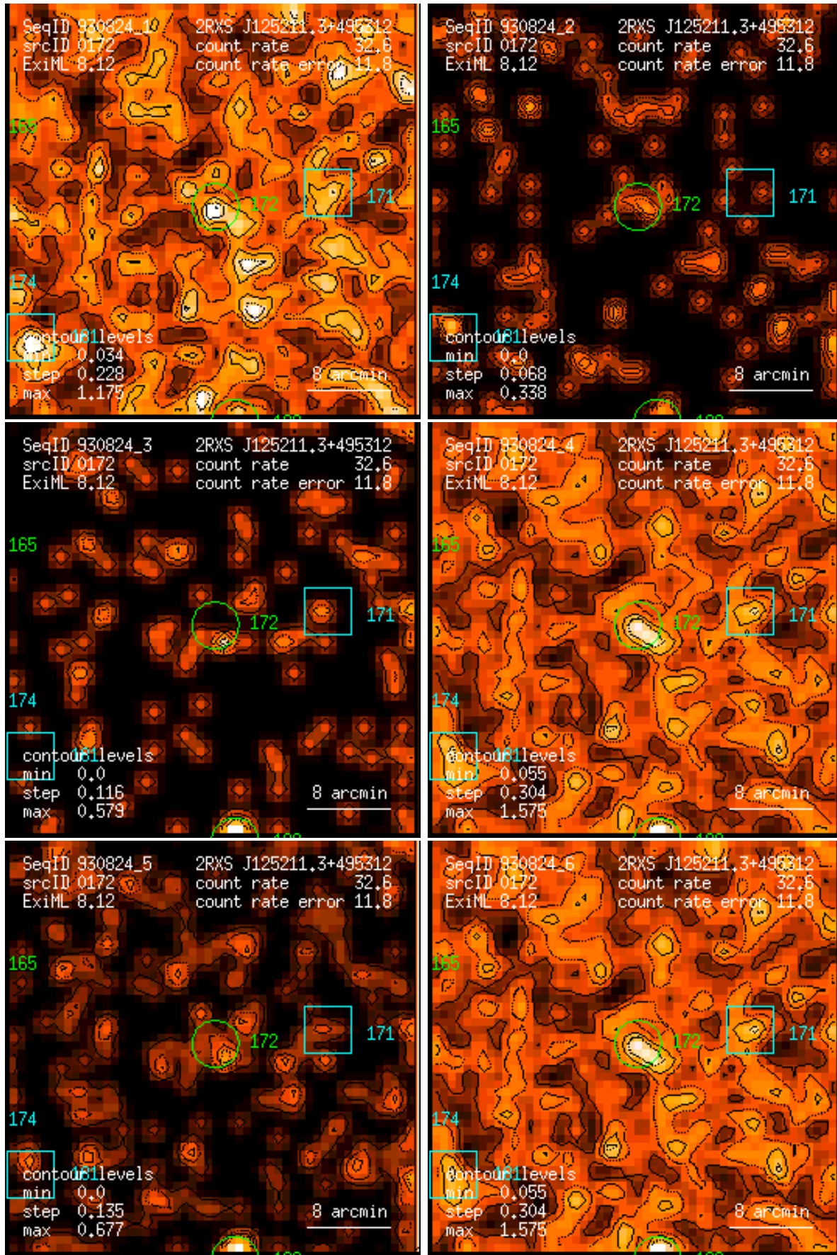
Figure 172: RASS 930824: detection 0172: band rate images, Gaussian filter: (1) PSPC channels 11 – 41, (2) 52 – 90, (3) 91 – 201, (4) 11 – 235, (5) 52 – 201, (6) 11 – 201. Broad band rates in counts/ks. Band rate contour levels in counts/ks/arcmin 2 .
