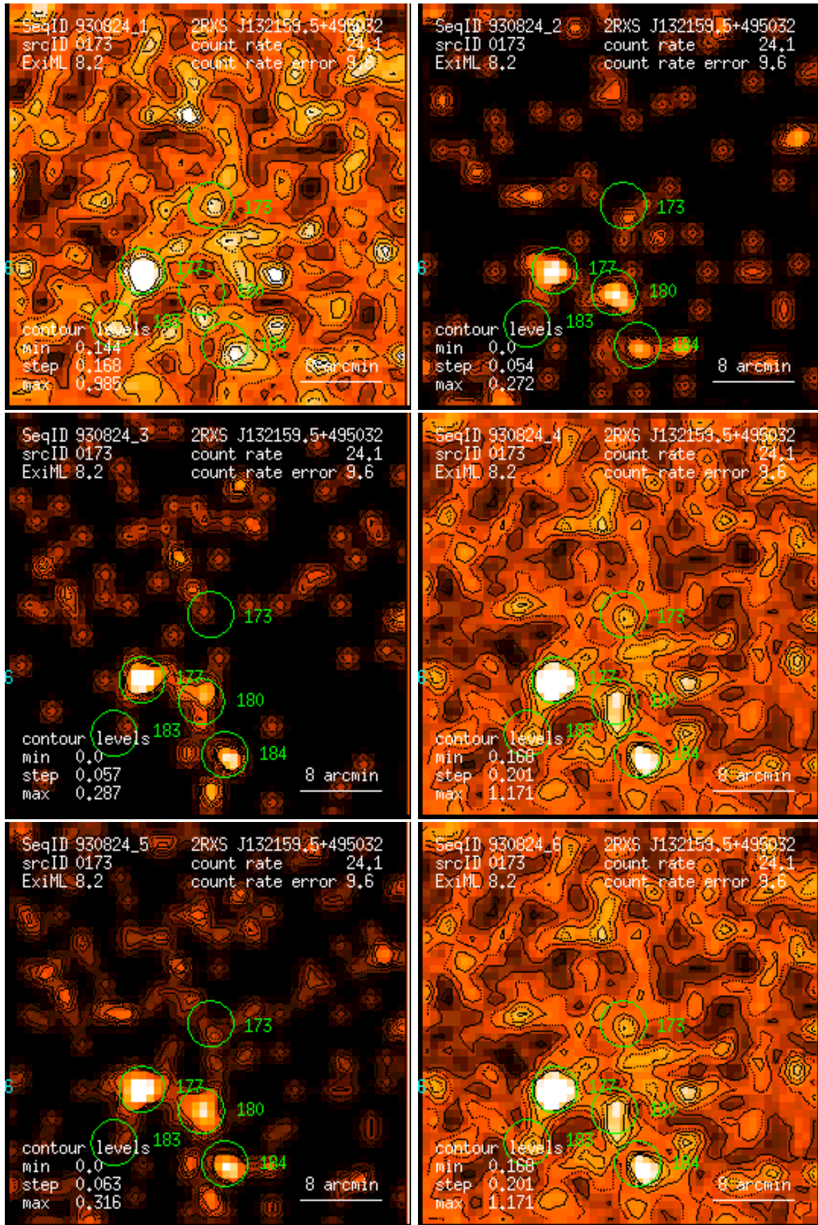
Figure 173: RASS 930824: detection 0173: band rate images, Gaussian filter: (1) PSPC channels 11 – 41, (2) 52 – 90, (3) 91 – 201, (4) 11 – 235, (5) 52 – 201, (6) 11 – 201. Broad band rates in counts/ks. Band rate contour levels in counts/ks/arcmin 2 .
