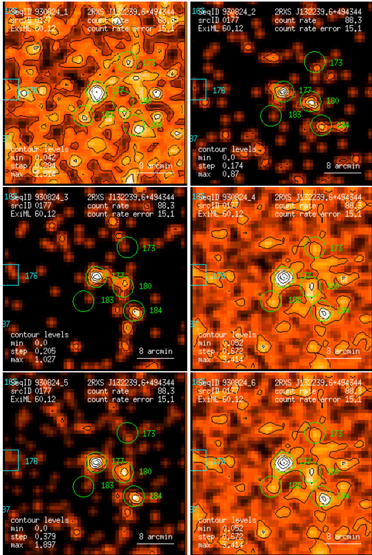
Figure 177: RASS 930824: detection 0177: band rate images, Gaussian filter: (1) PSPC channels 11 – 41, (2) 52 – 90, (3) 91 – 201, (4) 11 – 235, (5) 52 – 201, (6) 11 – 201. Broad band rates in counts/ks. Band rate contour levels in counts/ks/arcmin 2 .
