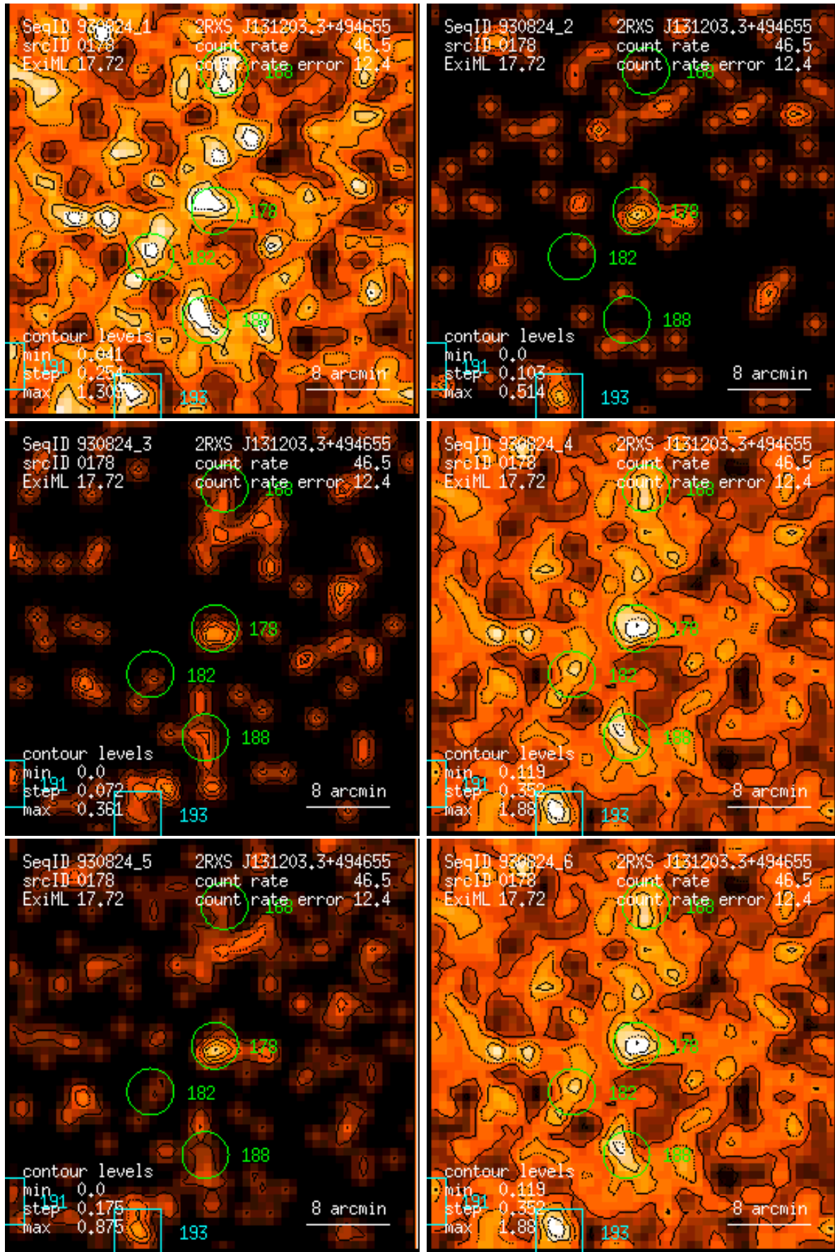
Figure 178: RASS 930824: detection 0178: band rate images, Gaussian filter: (1) PSPC channels 11 – 41, (2) 52 – 90, (3) 91 – 201, (4) 11 – 235, (5) 52 – 201, (6) 11 – 201. Broad band rates in counts/ks. Band rate contour levels in counts/ks/arcmin 2 .
