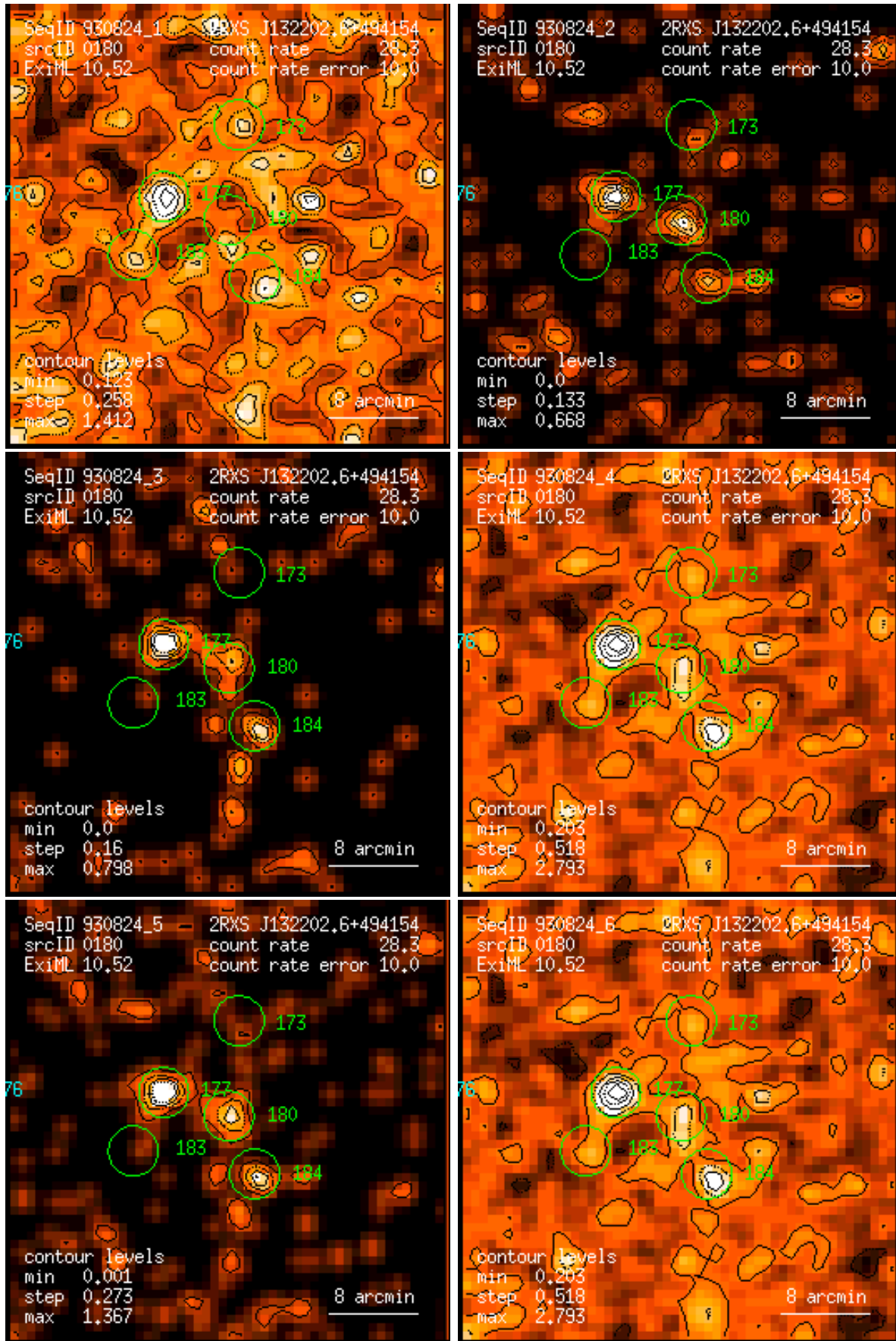
Figure 180: RASS 930824: detection 0180: band rate images, Gaussian filter: (1) PSPC channels 11 – 41, (2) 52 – 90, (3) 91 – 201, (4) 11 – 235, (5) 52 – 201, (6) 11 – 201. Broad band rates in counts/ks. Band rate contour levels in counts/ks/arcmin 2 .
