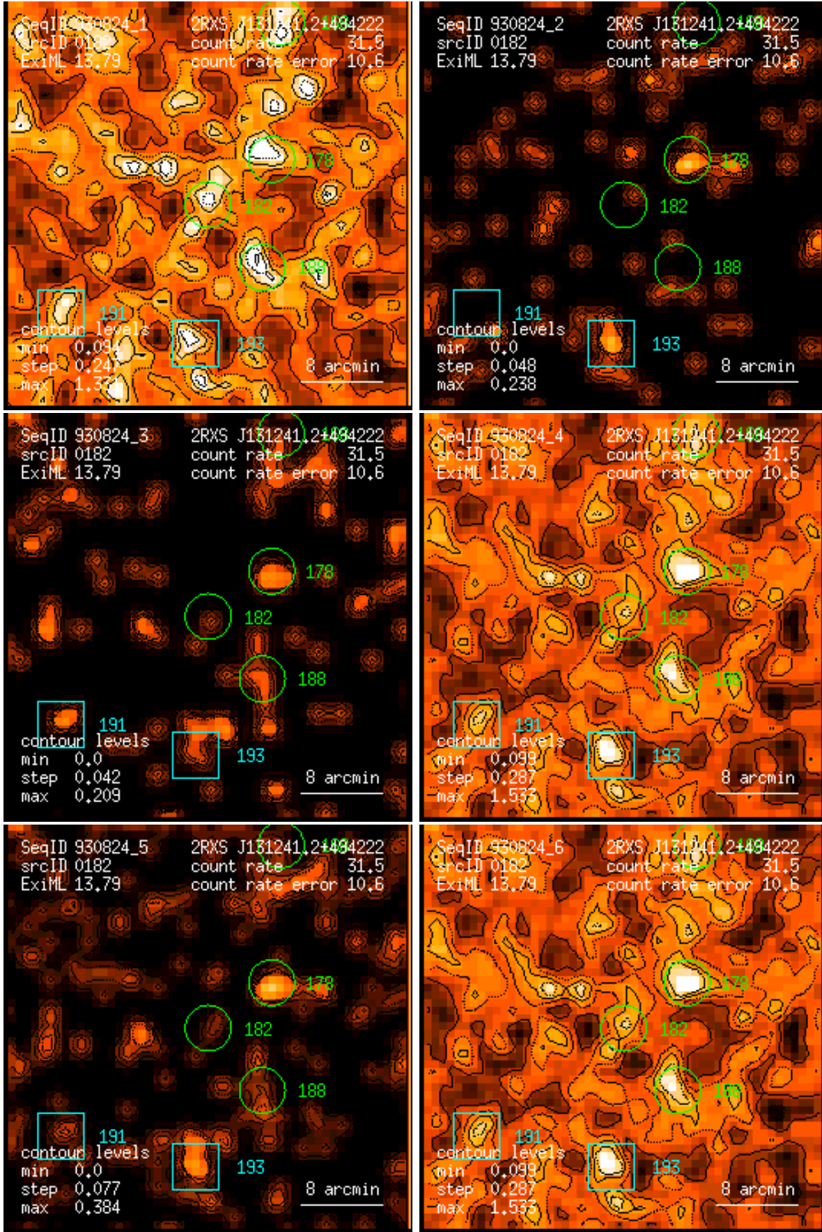
Figure 182: RASS 930824: detection 0182: band rate images, Gaussian filter: (1) PSPC channels 11 – 41, (2) 52 – 90, (3) 91 – 201, (4) 11 – 235, (5) 52 – 201, (6) 11 – 201. Broad band rates in counts/ks. Band rate contour levels in counts/ks/arcmin 2 .
