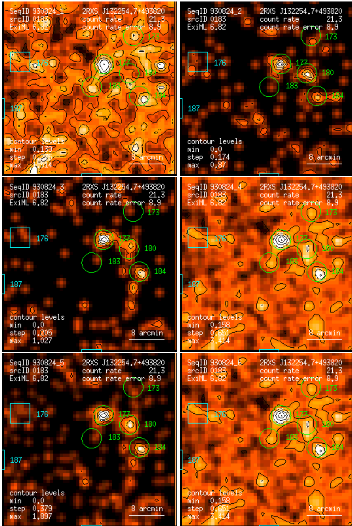
Figure 183: RASS 930824: detection 0183: band rate images, Gaussian filter: (1) PSPC channels 11 – 41, (2) 52 – 90, (3) 91 – 201, (4) 11 – 235, (5) 52 – 201, (6) 11 – 201. Broad band rates in counts/ks. Band rate contour levels in counts/ks/arcmin 2 .
