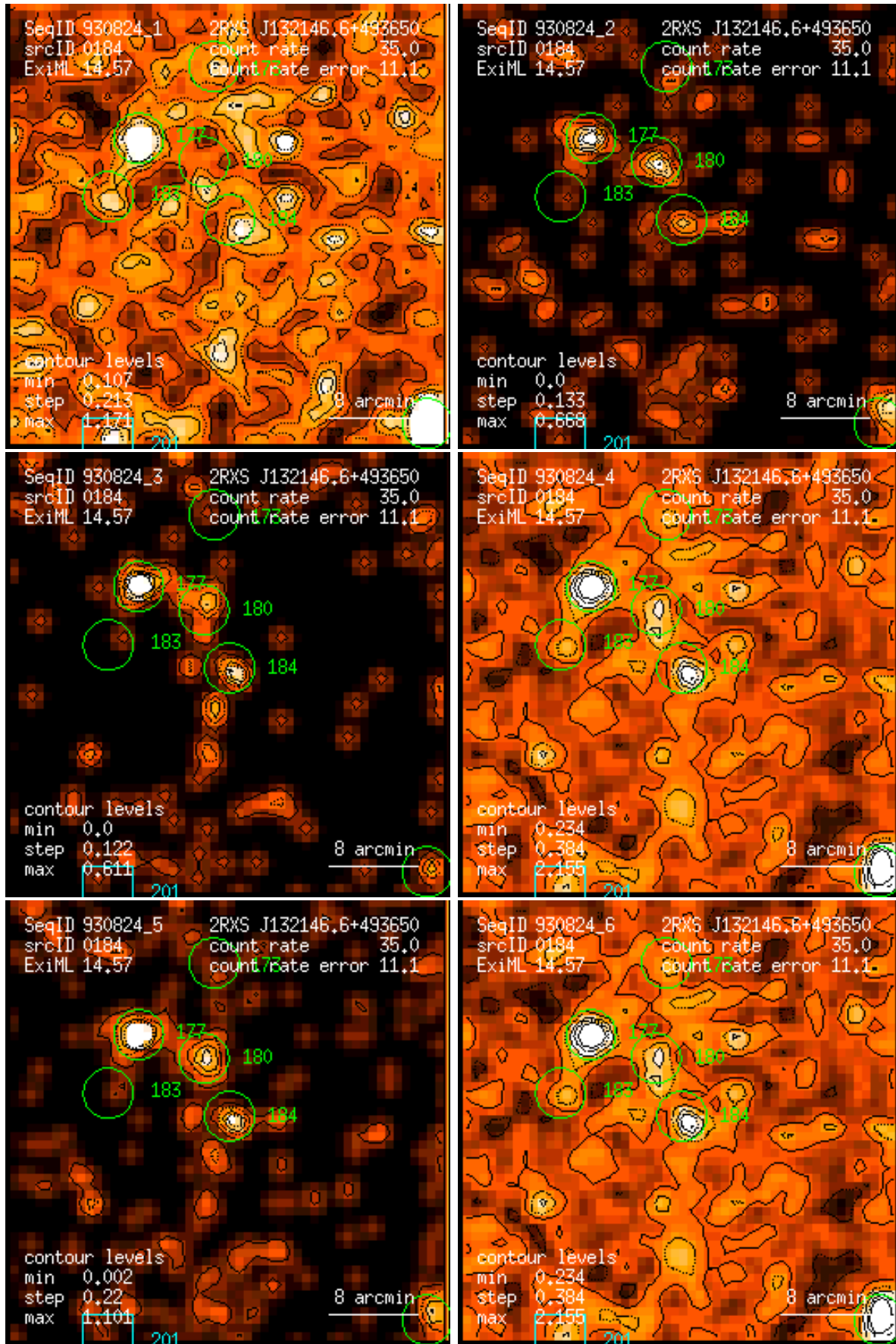
Figure 184: RASS 930824: detection 0184: band rate images, Gaussian filter: (1) PSPC channels 11 – 41, (2) 52 – 90, (3) 91 – 201, (4) 11 – 235, (5) 52 – 201, (6) 11 – 201. Broad band rates in counts/ks. Band rate contour levels in counts/ks/arcmin 2 .
