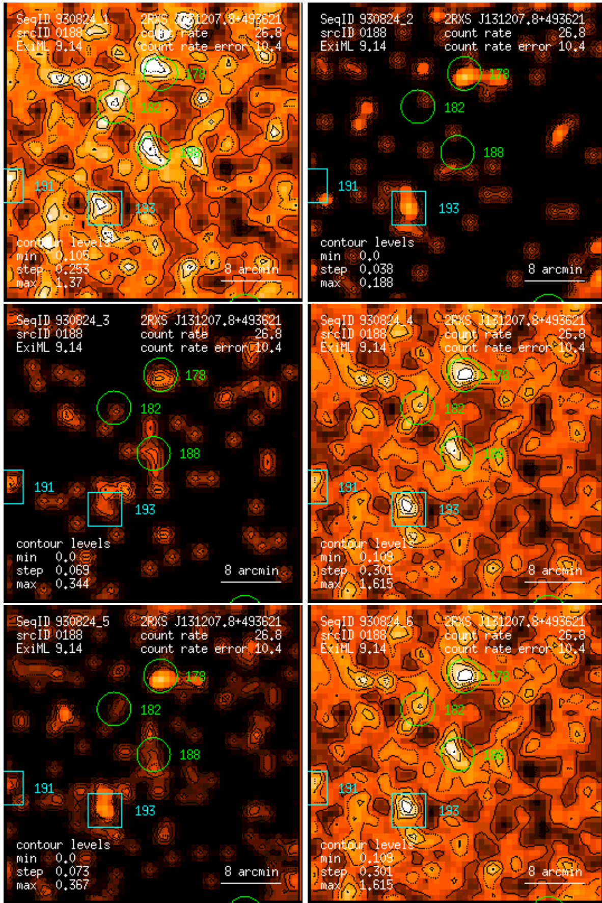
Figure 188: RASS 930824: detection 0188: band rate images, Gaussian filter: (1) PSPC channels 11 – 41, (2) 52 – 90, (3) 91 – 201, (4) 11 – 235, (5) 52 – 201, (6) 11 – 201. Broad band rates in counts/ks. Band rate contour levels in counts/ks/arcmin 2 .
