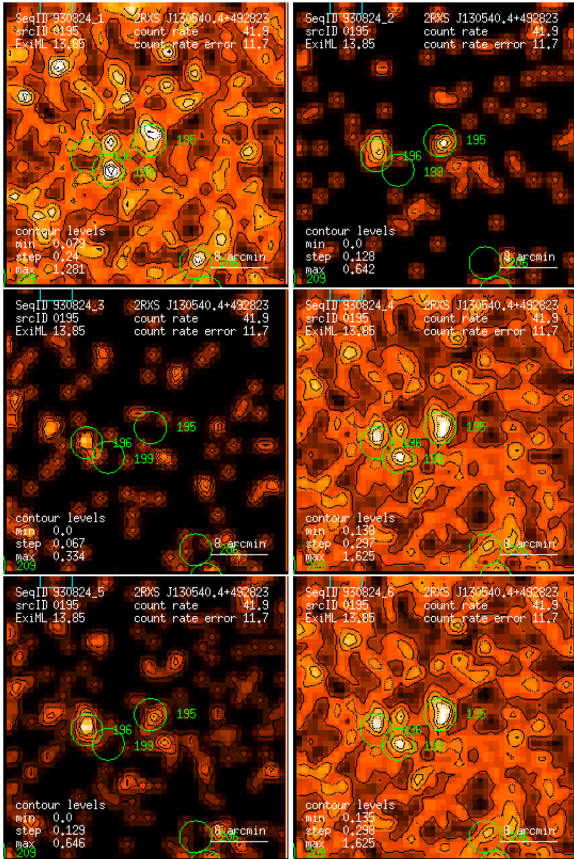
Figure 195: RASS 930824: detection 0195: band rate images, Gaussian filter: (1) PSPC channels 11 – 41, (2) 52 – 90, (3) 91 – 201, (4) 11 – 235, (5) 52 – 201, (6) 11 – 201. Broad band rates in counts/ks. Band rate contour levels in counts/ks/arcmin 2 .
