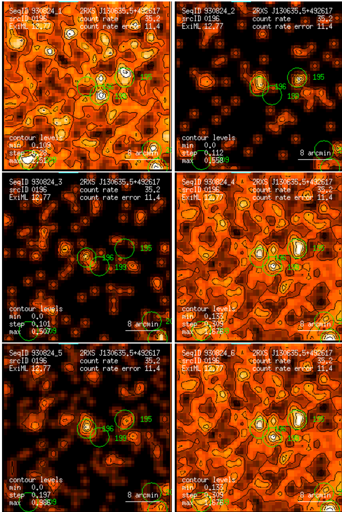
Figure 196: RASS 930824: detection 0196: band rate images, Gaussian filter: (1) PSPC channels 11 – 41, (2) 52 – 90, (3) 91 – 201, (4) 11 – 235, (5) 52 – 201, (6) 11 – 201. Broad band rates in counts/ks. Band rate contour levels in counts/ks/arcmin 2 .
