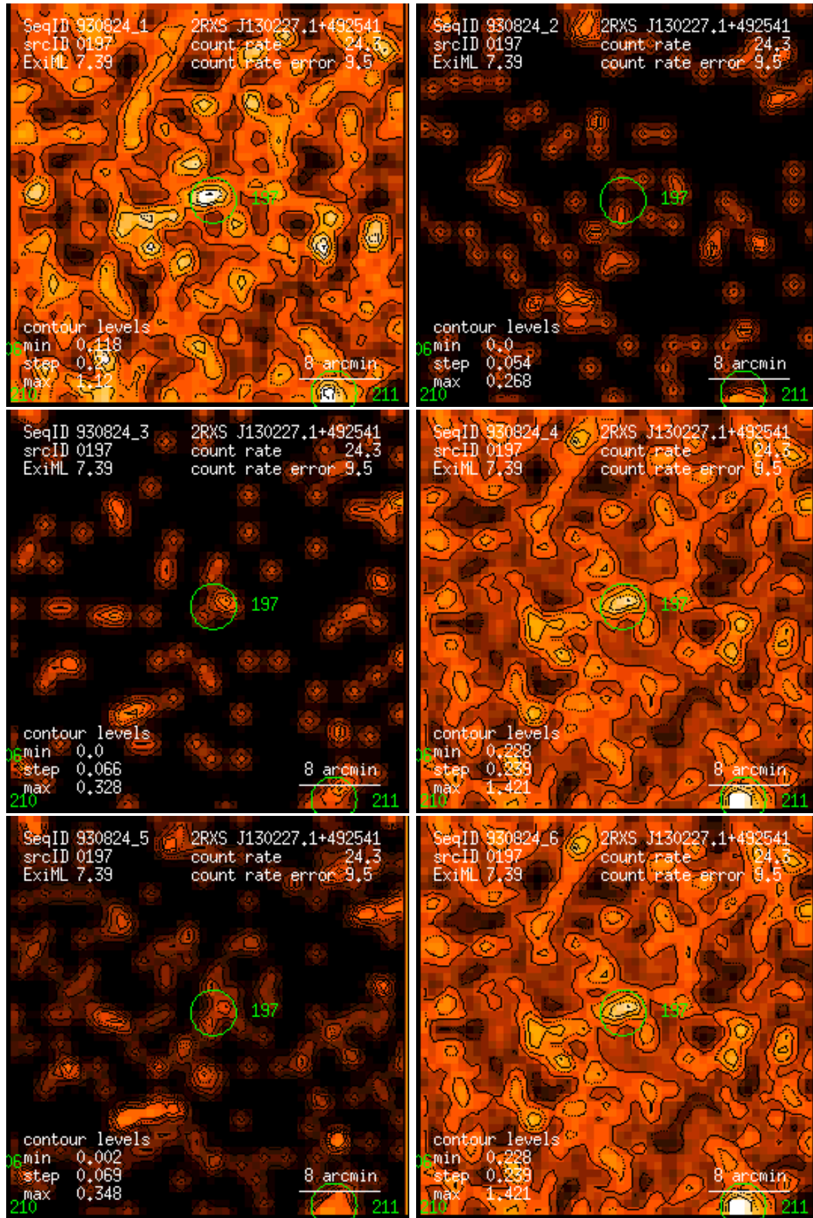
Figure 197: RASS 930824: detection 0197: band rate images, Gaussian filter: (1) PSPPC channels 11 – 41, (2) 52 – 90, (3) 91 – 201, (4) 11 – 235, (5) 52 – 201, (6) 11 – 201. Broad band rates in counts/ks. Band rate contour levels in counts/ks/arcmin 2 .
