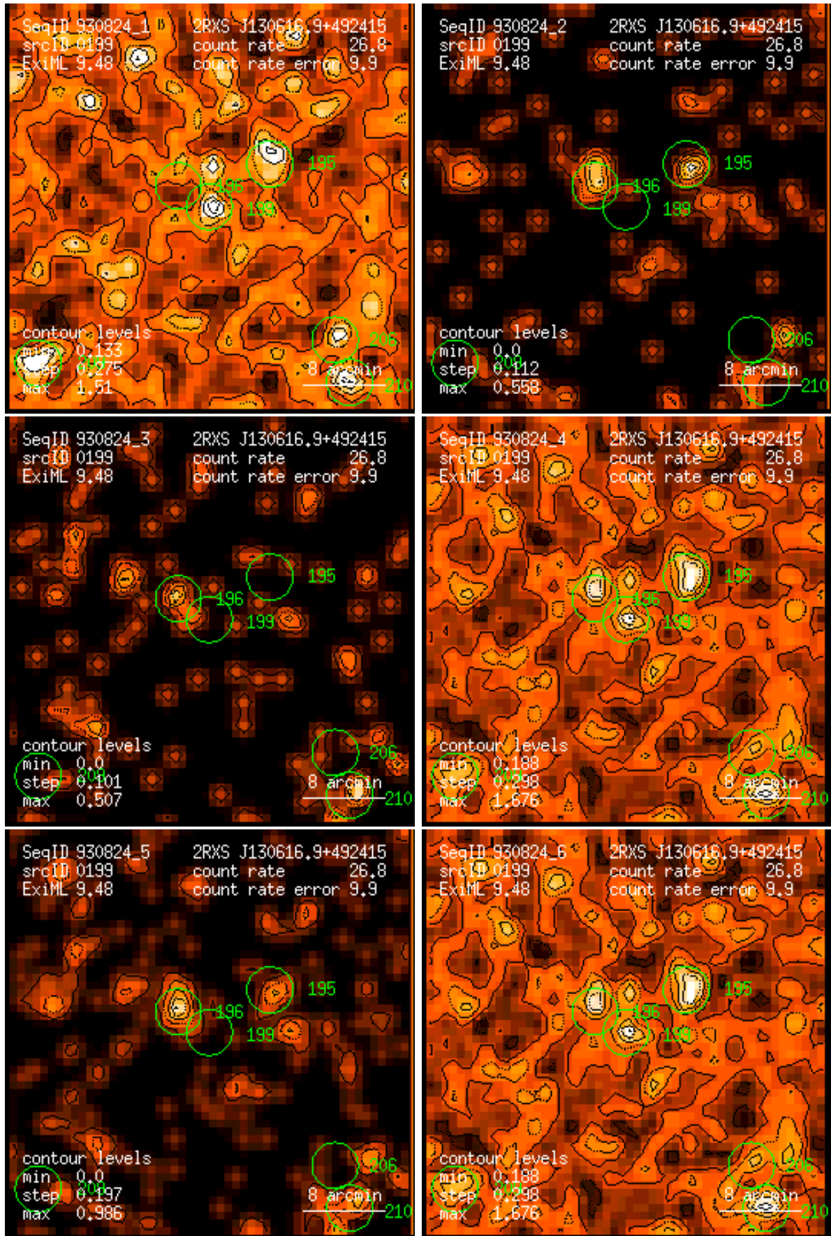
Figure 199: RASS 930824: detection 0199: band rate images, Gaussian filter: (1) PSPC channels 11 – 41, (2) 52 – 90, (3) 91 – 201, (4) 11 – 235, (5) 52 – 201, (6) 11 – 201. Broad band rates in counts/ks. Band rate contour levels in counts/ks/arcmin 2 .
