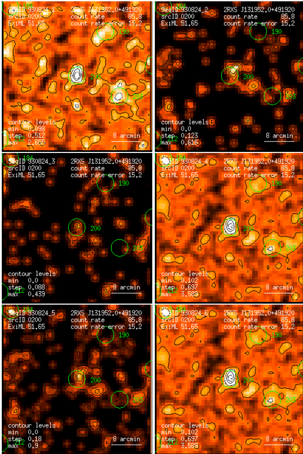
Figure 200: RASS 930824: detection 0200: band rate images, Gaussian filter: (1) PSPC channels 11 – 41, (2) 52 – 90, (3) 91 – 201, (4) 11 – 235, (5) 52 – 201, (6) 11 – 201. Broad band rates in counts/ks. Band rate contour levels in counts/ks/arcmin 2 .
