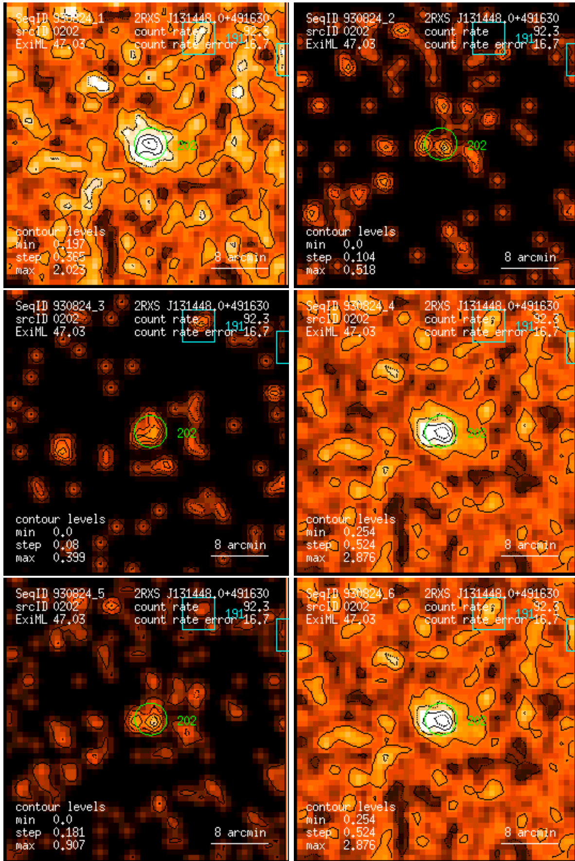
Figure 202: RASS 930824: detection 0202: band rate images, Gaussian filter: (1) PSPC channels 11 – 41, (2) 52 – 90, (3) 91 – 201, (4) 11 – 235, (5) 52 – 201, (6) 11 – 201. Broad band rates in counts/ks. Band rate contour levels in counts/ks/arcmin 2 .
