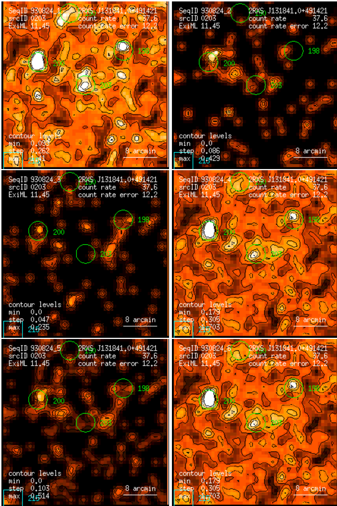
Figure 203: RASS 930824: detection 0203: band rate images, Gaussian filter: (1) PSPC channels 11 – 41, (2) 52 – 90, (3) 91 – 201, (4) 11 – 235, (5) 52 – 201, (6) 11 – 201. Broad band rates in counts/ks. Band rate contour levels in counts/ks/arcmin 2 .
