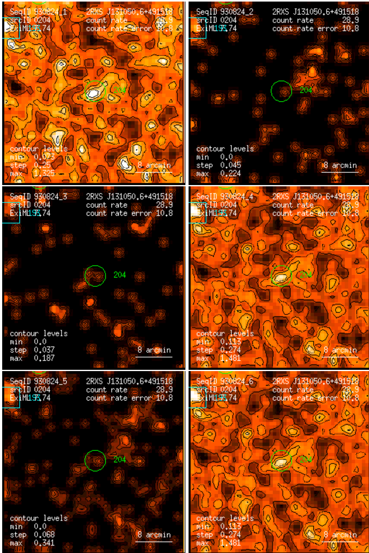
Figure 204: RASS 930824: detection 0204: band rate images, Gaussian filter: (1) PSPC channels 11 – 41, (2) 52 – 90, (3) 91 – 201, (4) 11 – 235, (5) 52 – 201, (6) 11 – 201. Broad band rates in counts/ks. Band rate contour levels in counts/ks/arcmin 2 .
