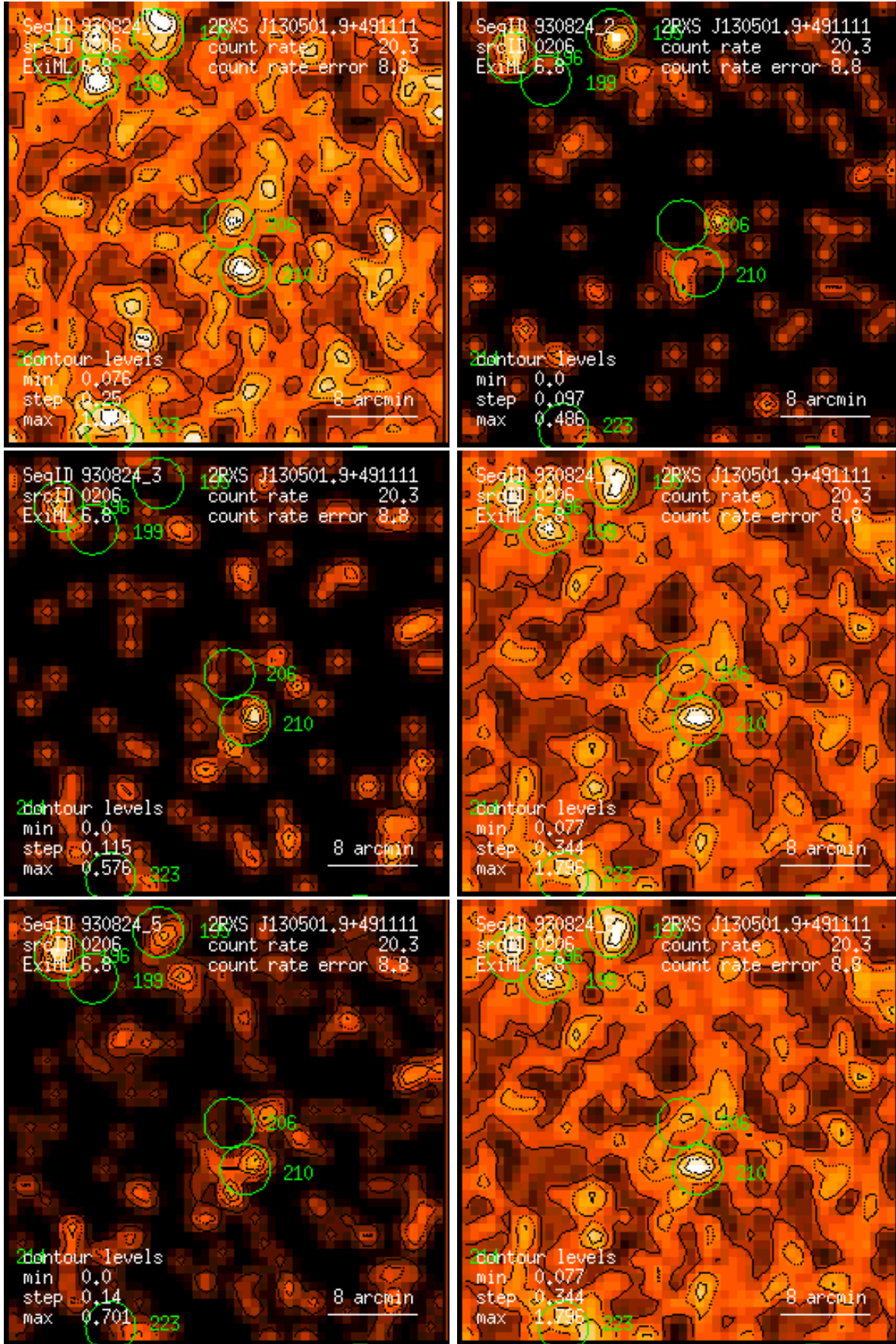
Figure 206: RASS 930824: detection 0206: band rate images, Gaussian filter: (1) PSPC channels 11 – 41, (2) 52 – 90, (3) 91 – 201, (4) 11 – 235, (5) 52 – 201, (6) 11 – 201. Broad band rates in counts/ks. Band rate contour levels in counts/ks/arcmin 2 .
