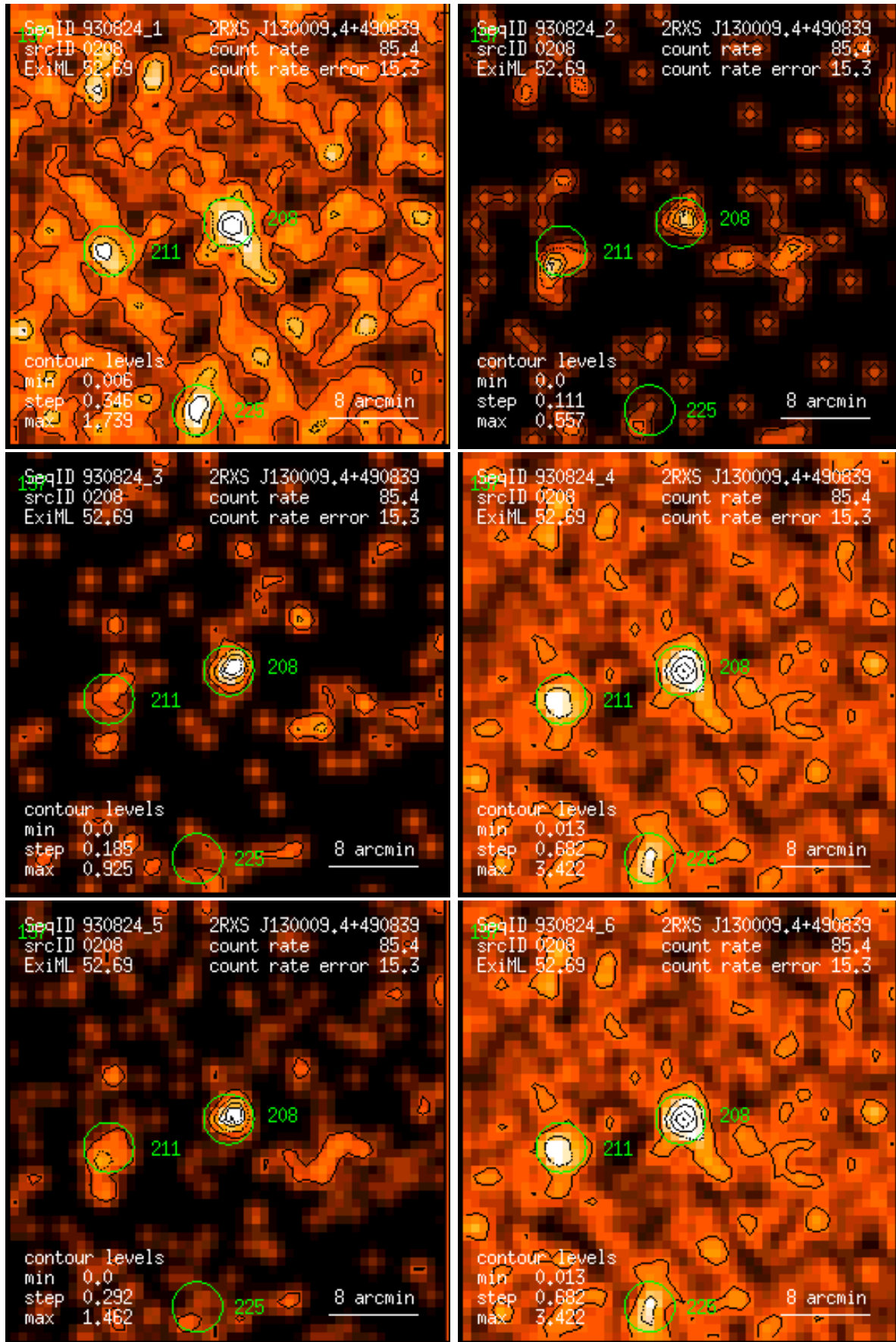
Figure 208: RASS 930824: detection 0208: band rate images, Gaussian filter: (1) PSPC channels 11 – 41, (2) 52 – 90, (3) 91 – 201, (4) 11 – 235, (5) 52 – 201, (6) 11 – 201. Broad band rates in counts/ks. Band rate contour levels in counts/ks/arcmin 2 .
