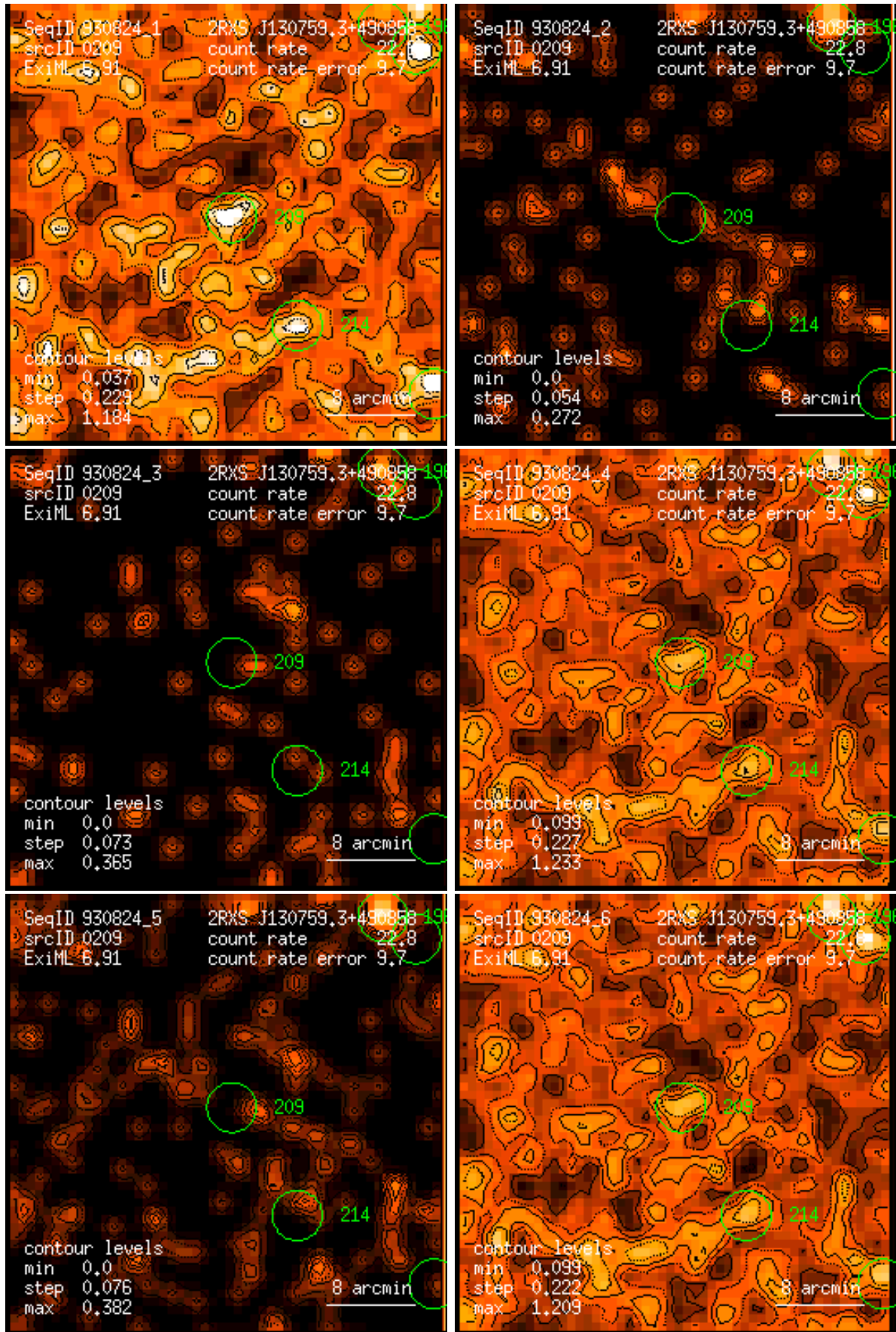
Figure 209: RASS 930824: detection 0209: band rate images, Gaussian filter: (1) PSPC channels 11 – 41, (2) 52 – 90, (3) 91 – 201, (4) 11 – 235, (5) 52 – 201, (6) 11 – 201. Broad band rates in counts/ks. Band rate contour levels in counts/ks/arcmin 2 .
