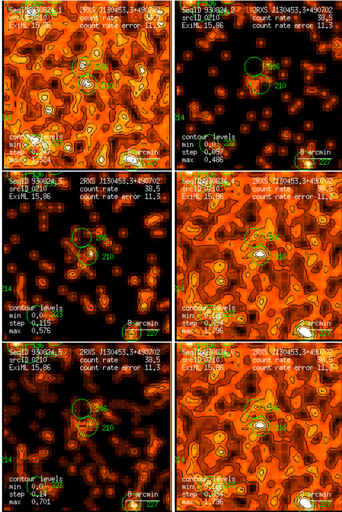
Figure 210: RASS 930824: detection 0210: band rate images, Gaussian filter: (1) PSPC channels 11 – 41, (2) 52 – 90, (3) 91 – 201, (4) 11 – 235, (5) 52 – 201, (6) 11 – 201. Broad band rates in counts/ks. Band rate contour levels in counts/ks/arcmin 2 .
