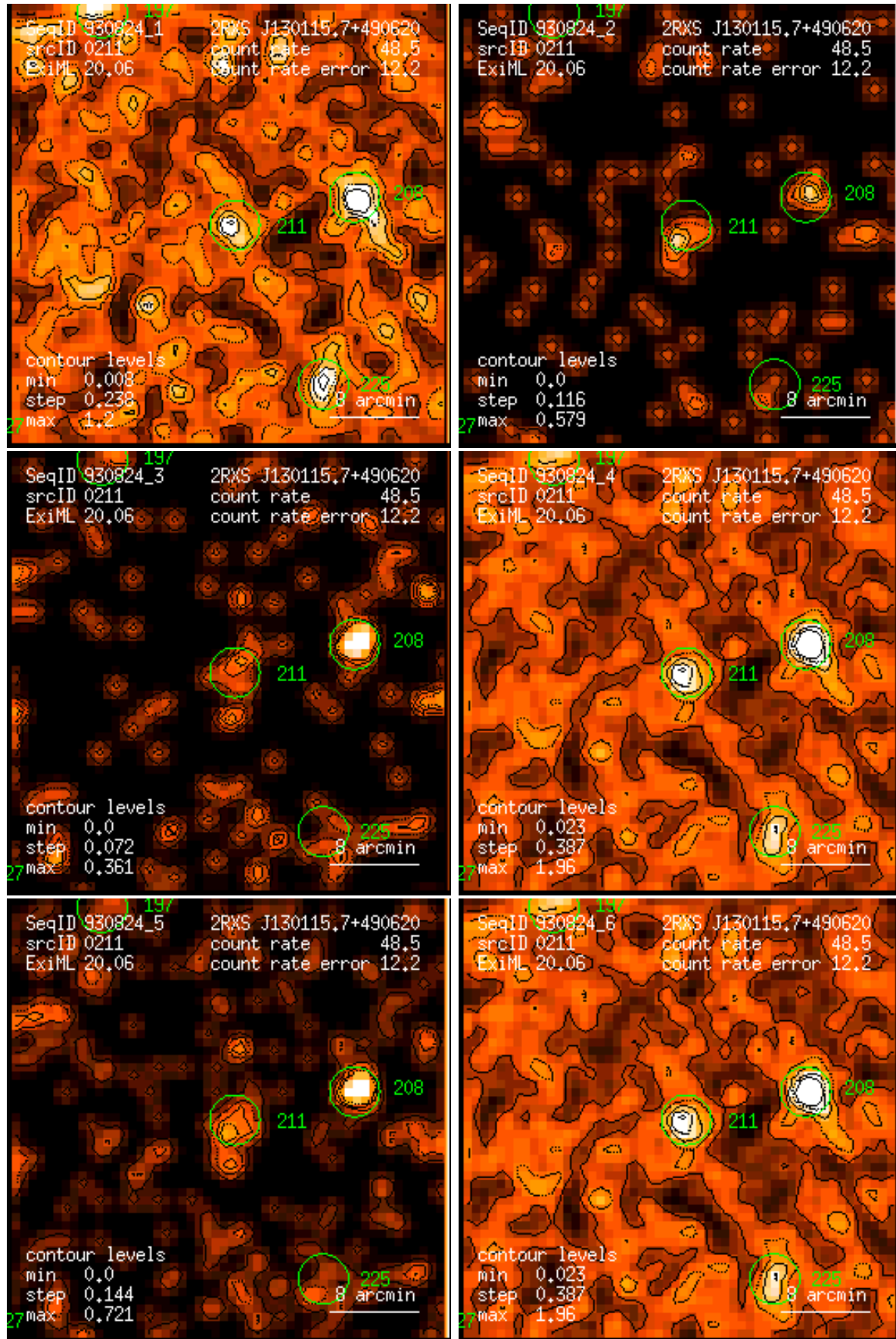
Figure 211: RASS 930824: detection 0211: band rate images, Gaussian filter: (1) PSPC channels 11 – 41, (2) 52 – 90, (3) 91 – 201, (4) 11 – 235, (5) 52 – 201, (6) 11 – 201. Broad band rates in counts/ks. Band rate contour levels in counts/ks/arcmin 2 .
