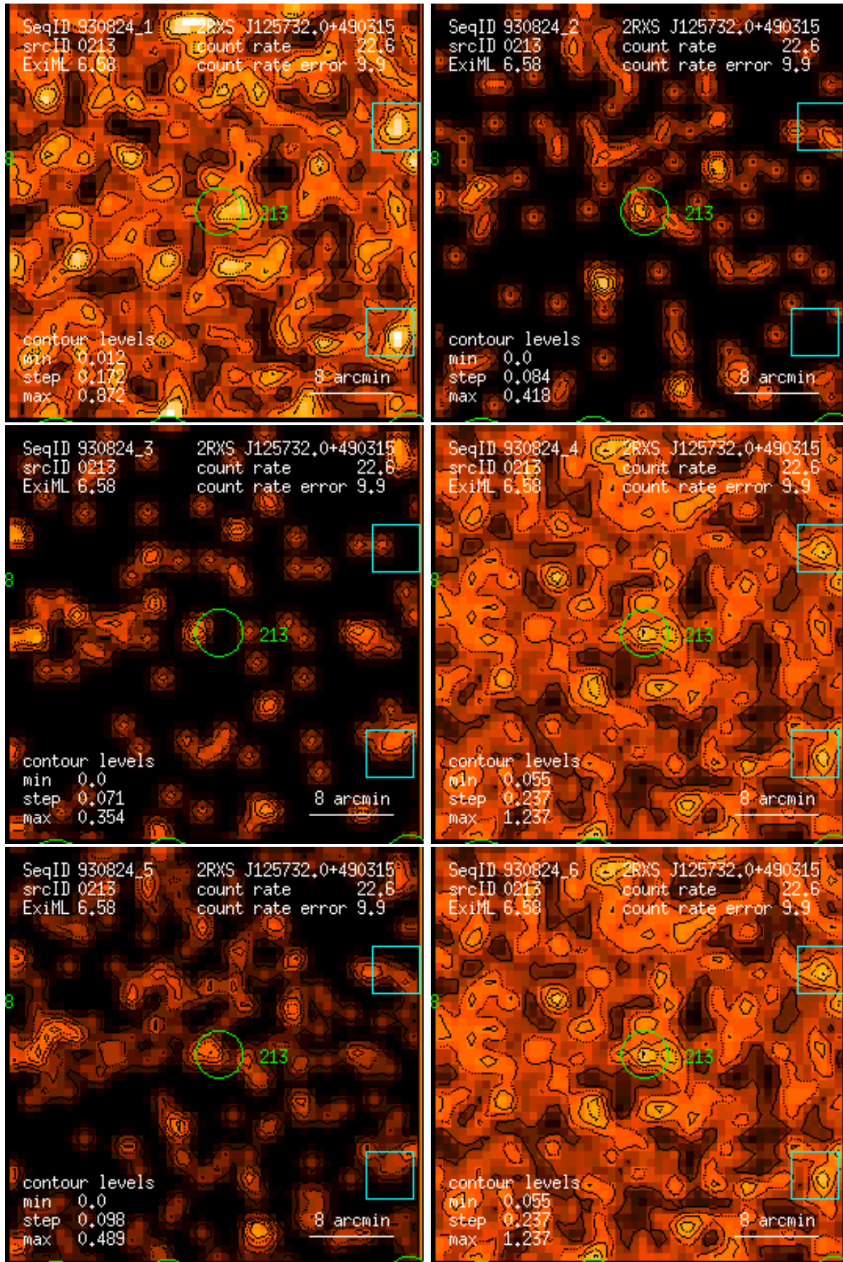
Figure 213: RASS 930824: detection 0213: band rate images, Gaussian filter: (1) PSPC channels 11 – 41, (2) 52 – 90, (3) 91 – 201, (4) 11 – 235, (5) 52 – 201, (6) 11 – 201. Broad band rates in counts/ks. Band rate contour levels in counts/ks/arcmin 2 .
